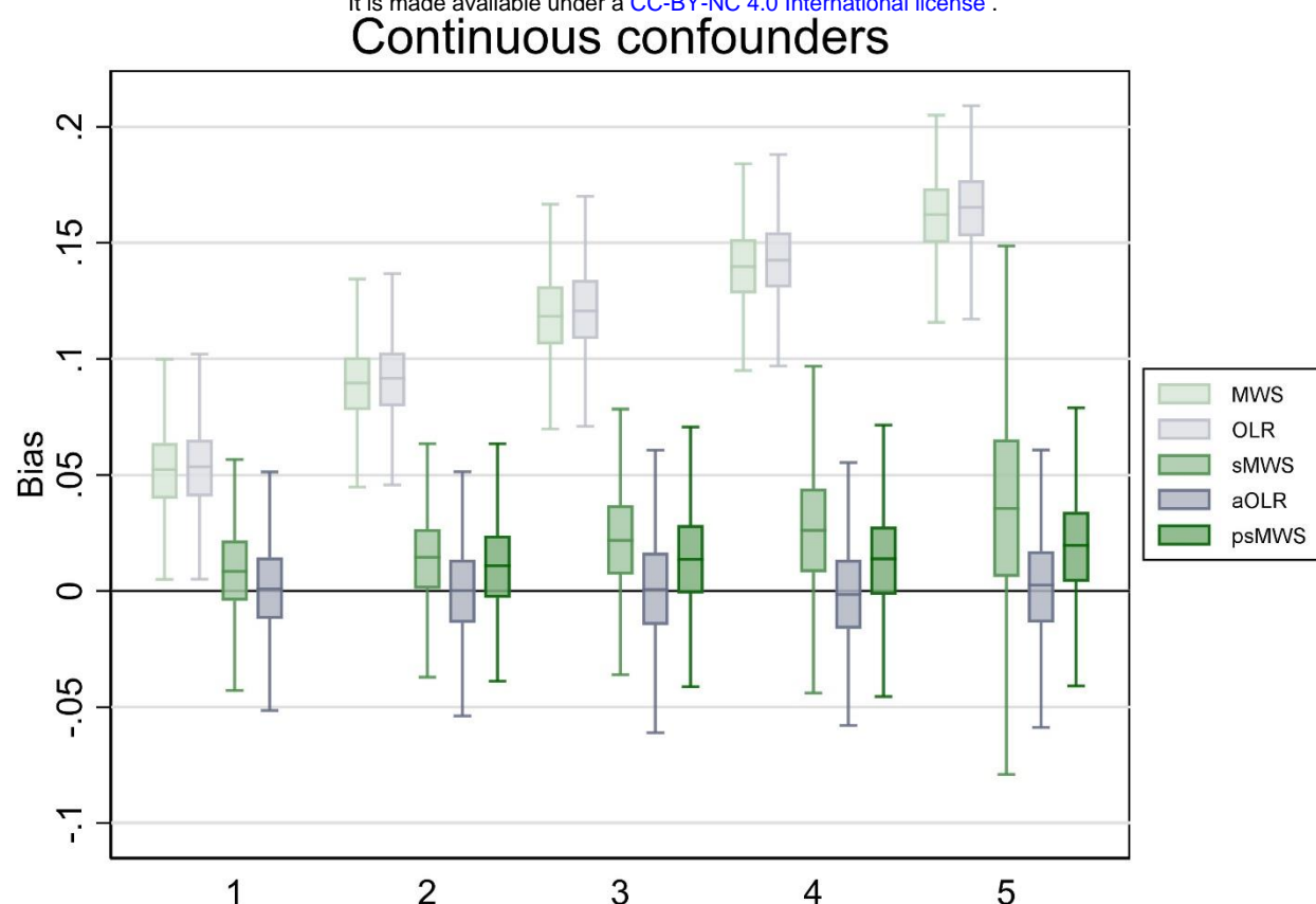
Figure 2. Bias of Mann-Whitney measure of superiority (MWS), ordinal logistic regression (OLR), stratified Mann-Whitney measure of superiority (sMWS), adjusted ordinal logistic regression (aOLR), and propensity score based stratified Mann-Whitney measure of superiority (psMWS) in scenario 2. The psMWS was not performed in the scenario with one confounding variable. Runs (N): 1000.
