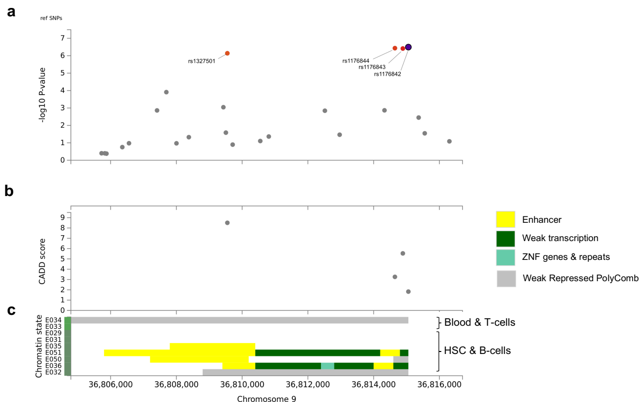
Suppl. Figure 7. Putative regulatory effects of PAX5 locus variants. Genomic position is plotted against: (a) the negative common logarithm of the p-value from the fixed-effects meta-analysis; (b) the Combined Annotation Dependent Depletion (CADD) score, a scaled measure of pathogenicity in which scores of 10 and 20, respectively, indicate that a variant is among the most 10% and 1% deleterious in the human genome; [32] (c) the chromatin states of nine cell types annotated using the core 15-state state model (ChromHMM), which predicts regulatory annotations based on histone modifications. [33] E034, primary T-cells from peripheral blood; E033, primary T cells from cord blood; E029, primary monocytes from peripheral blood; E031, primary B cells from cord blood; E035, primary hematopoietic stem cells; E051, primary hematopoietic stem cells G-CSF-mobilised (male); E050, primary hematopoietic stem cells G-CSF-mobilised (female); E036, primary hematopoietic stem cells in short term culture; E032, primary B cells from peripheral blood. The plot was generated using the FUMA web application.[34]
