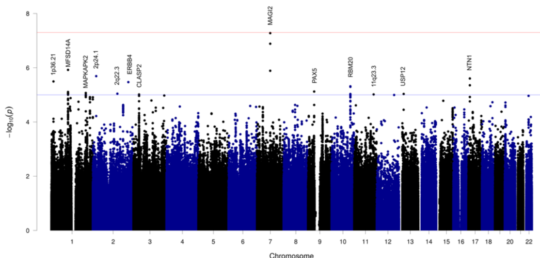
Suppl. Figure 6. Manhattan plot for the genome-wide meta-analysis. Directly genotyped and imputed variants at MAF greater than 5% were tested for association with invasive GAS susceptibility in all four case-control analyses using linear mixed models. The association statistics were combined by (a) fixed-effects or (b) random-effects meta-analysis. Each point represents a single variant. The blue horizontal line indicates the suggestive significance threshold ( P = 10^{-5} ) and the red horizontal line indicates the genome-wide significance threshold ( P = 5 \times 10^{-8} ).
