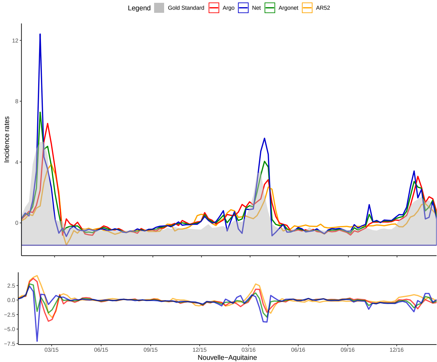
Fig 12. Nouvelle-Aquitaine Two-week ahead estimate
