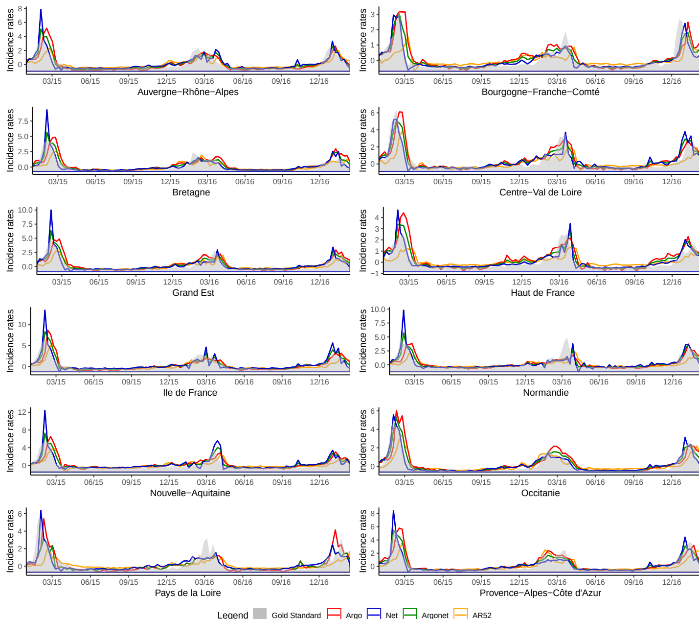
Fig 10. Two-week ahead estimate obtained with ARGO, Net and ARGONet models from January 2015 to March 2017
