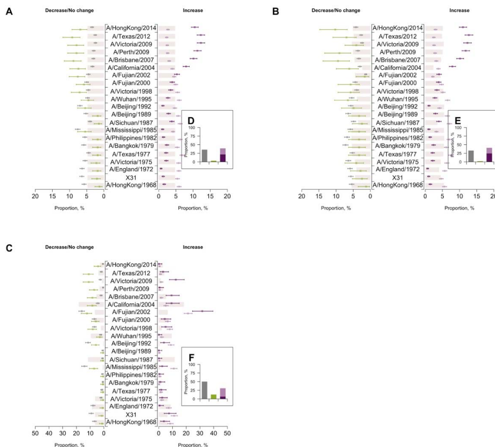
Fig. S15. Distribution of H3N2 strains by changes in titers between two visits.
