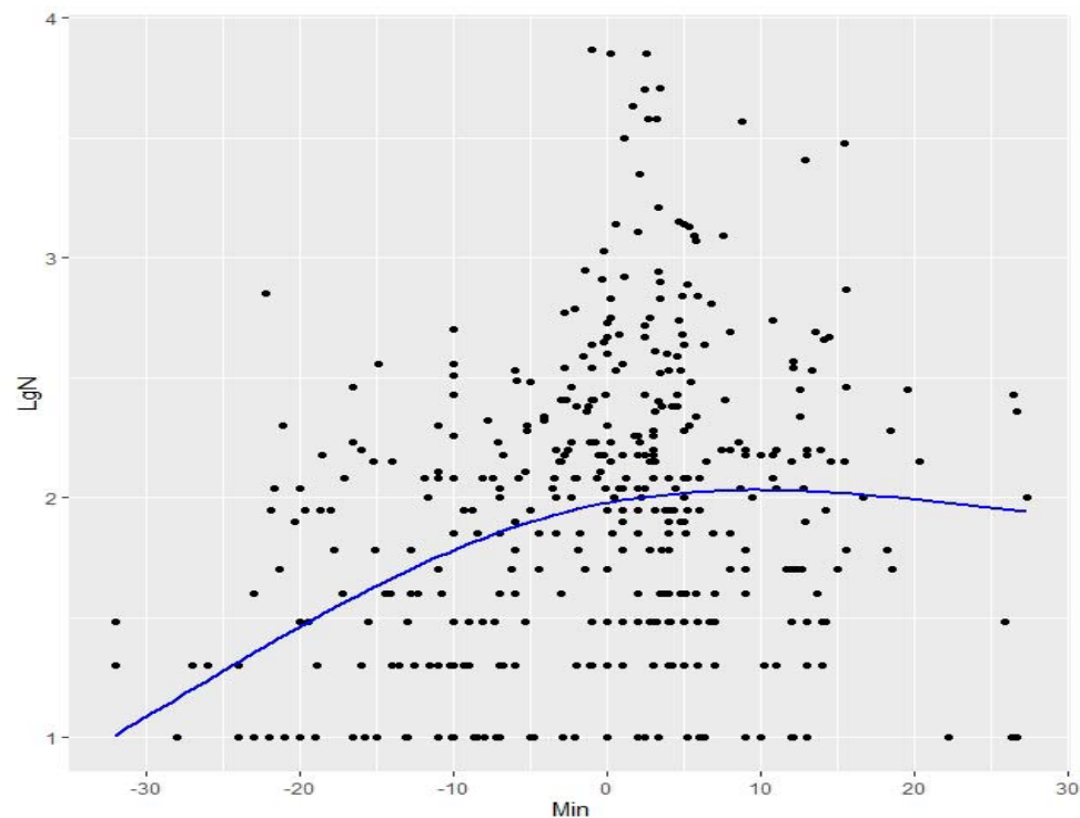
Figure 2b The cubic spline curve between minimum temperature and lgN of COVID-19 transmission in the world
