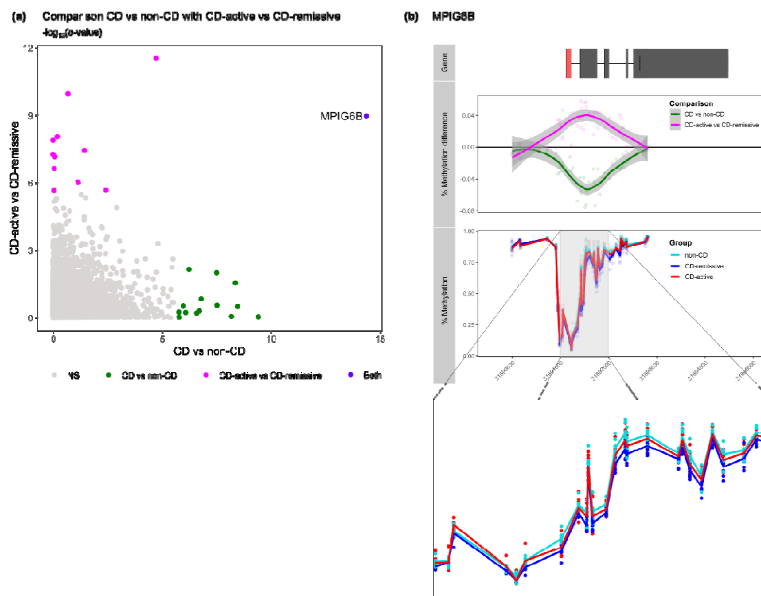
Figure 3. Comparison of the DMGs across the two comparisons. (a) Visualization of the Fisher's combined probability test p -values from CD vs non-CD on the x-axis and CD-active vs CD-remissive on the y-axis. Colors represent the genes found to be significant in the different comparisons. (b) Visualization of the percentage MPIG6B methylation for non-CD, CD-active and CD-remissive separately with an enlarged visualization below.
