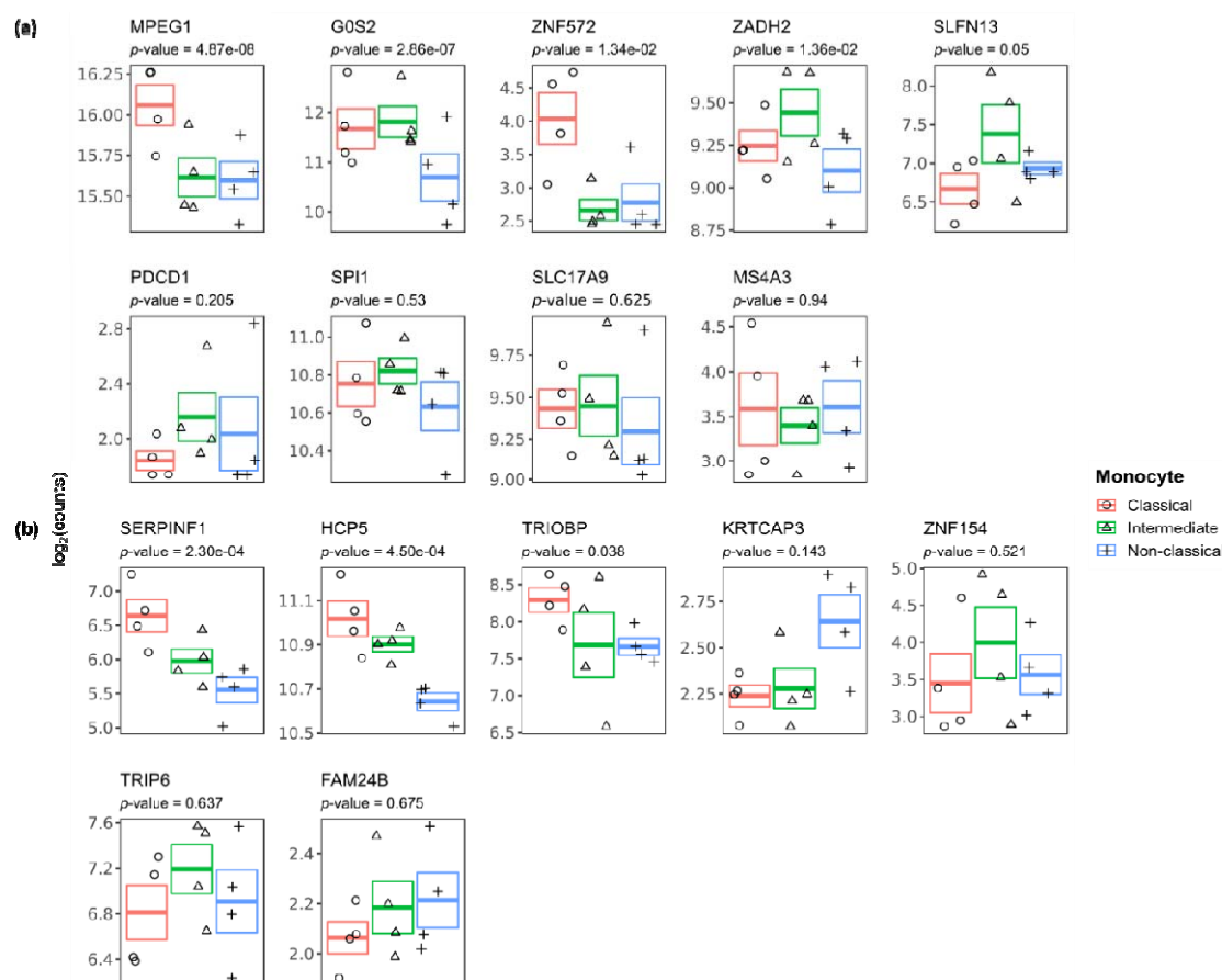
Figure 4. Gene expression of the DMGs across the different monocyte subsets. Visualization of the \log_2(\text{counts}) for classical, intermediate and non-classical annotated with the p -value as obtained from the likelihood ratio test.
