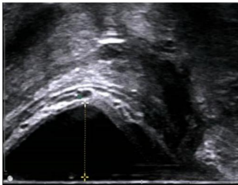
Figure 8:rectocele
