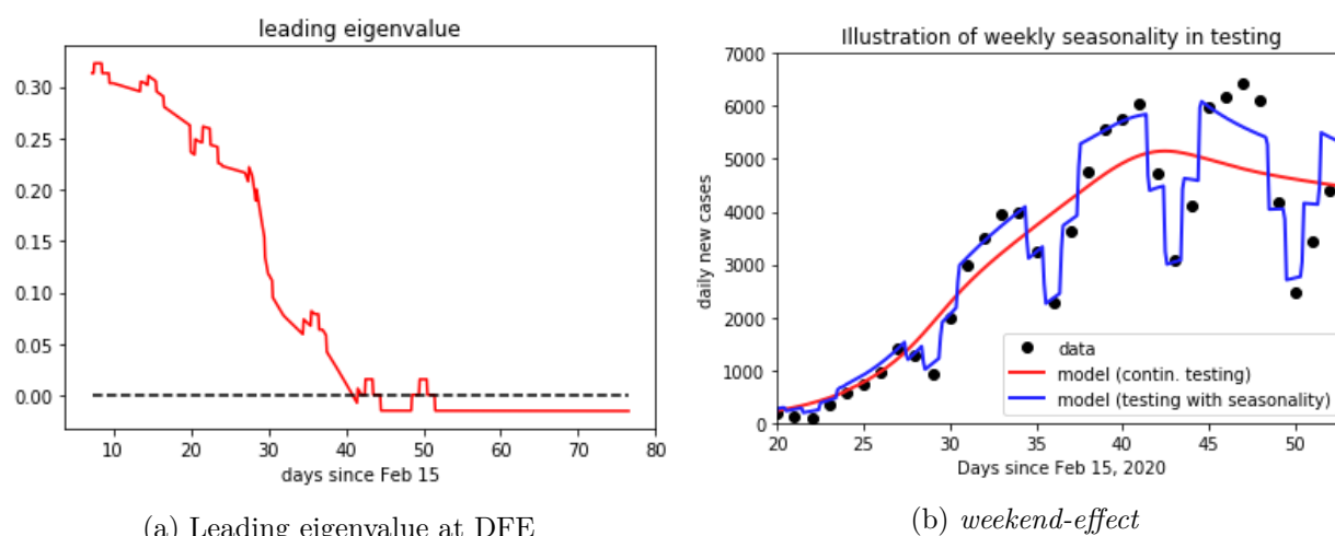
Figure 6: (a) Evolution in time of the dominant eigenvalue of linearization of the age and stage structured model at the disease free equilibrium (DFE). The dominant eigenvalue crossing the zero axis corresponds to the reproduction number crossing the threshold value 1. (b) The weekend effect accounting for fluctuations in case detection and reporting. Black dots denote daily reported new cases, continuous curves show the model solutions with (blue) and without (red) time-dependent testing rates.
