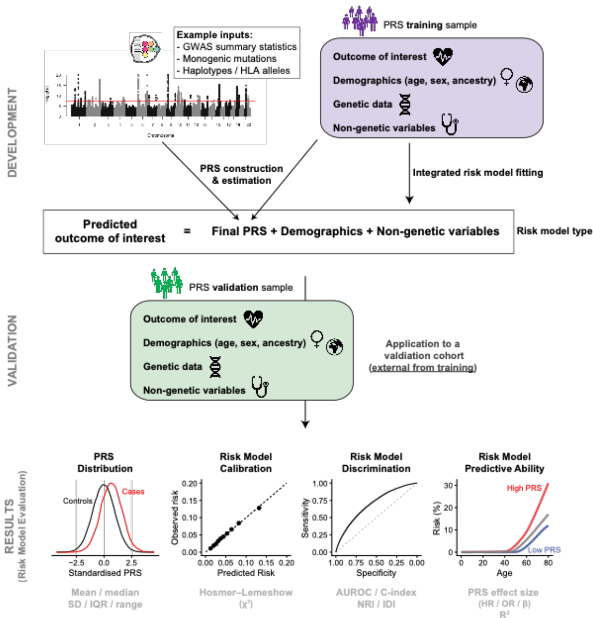
Figure 1: Prototype of PRS development and validation process. Figure 1 displays prototypical steps for PRS construction, risk model development, and validation of performance with select aspects of the PRS-RS guideline labeled in bold text throughout. In PRS development, variants associated with an outcome of interest, typically identified from a GWAS, are combined as a weighted sum of allele counts across variants. Methods for optimizing variant selection for a PRS (PRS construction & estimation) are not shown. The PRS is tested in a risk model predicting the outcome of interest and may be combined with other non-genetic variables (e.g. age, sex, ancestry, clinical variables); collectively these are referred to as risk model variables. After fitting procedures to select the best risk model, this model is validated in an independent sample. The PRS distribution should be described, and the performance of the risk model demonstrated in terms of its discrimination, predictive ability, and calibration. Though not displayed in the figure, these same results should also be reported for the training sample for comparison to the validation sample. In both training and validation cohorts, the outcome of interest criteria, demographics, genotyping, and non-genetic variables should be reported (Table 1).
