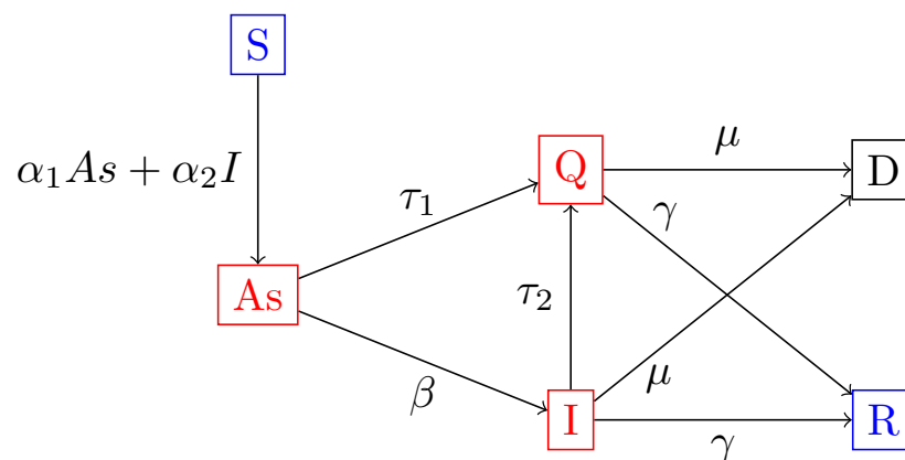
Figure 1: The model flow chart
