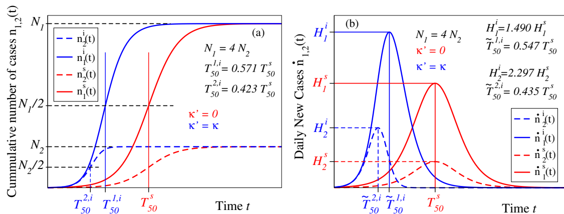
Figure 4: (a) Cumulative number of cases n_{1,2}(t) and (b) epidemiologic curves \dot{n}_{1,2}(t) \equiv dn_{1,2}(t)/dt for two completely separated and perfectly intermingled (red and blue curves, respectively) groups whose populations differ by a factor of four. Notice that, in spite of the equal infection rates, infection of the smaller group 2 (dashed lines) is stronger affected by the inter-group interaction than in the larger group 1 (solid lines). Time on the x -axis is expressed in units of the characteristic time T_c = \kappa^{-1} .
