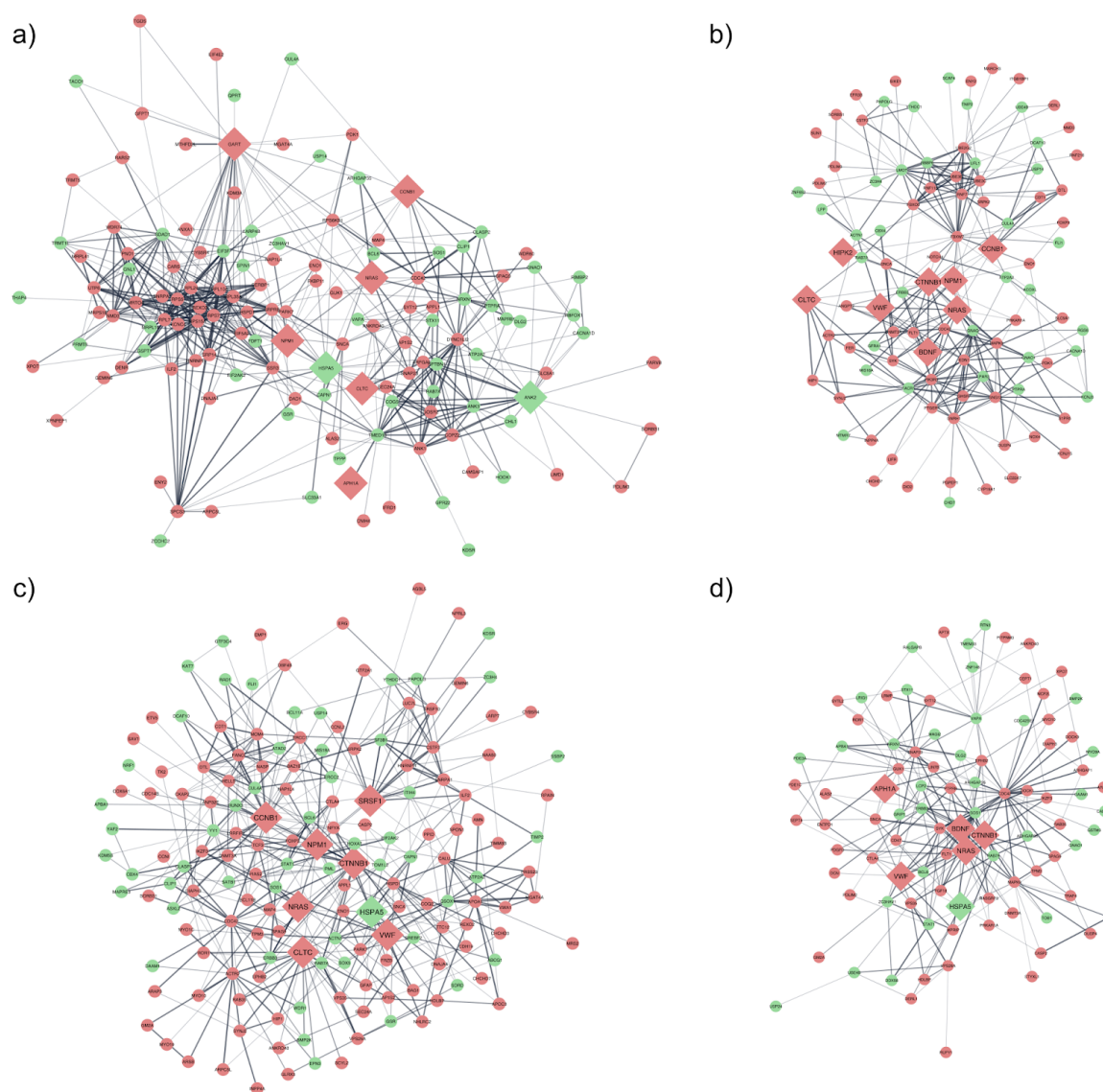
Fig. 2 The four modules with the highest score identified by MCODE in the PPI network. Green nodes denote down-regulated genes in AF, whereas red nodes represent up-regulated genes. Diamond nodes indicate hub-bottlenecks identified in the network structural analysis.
