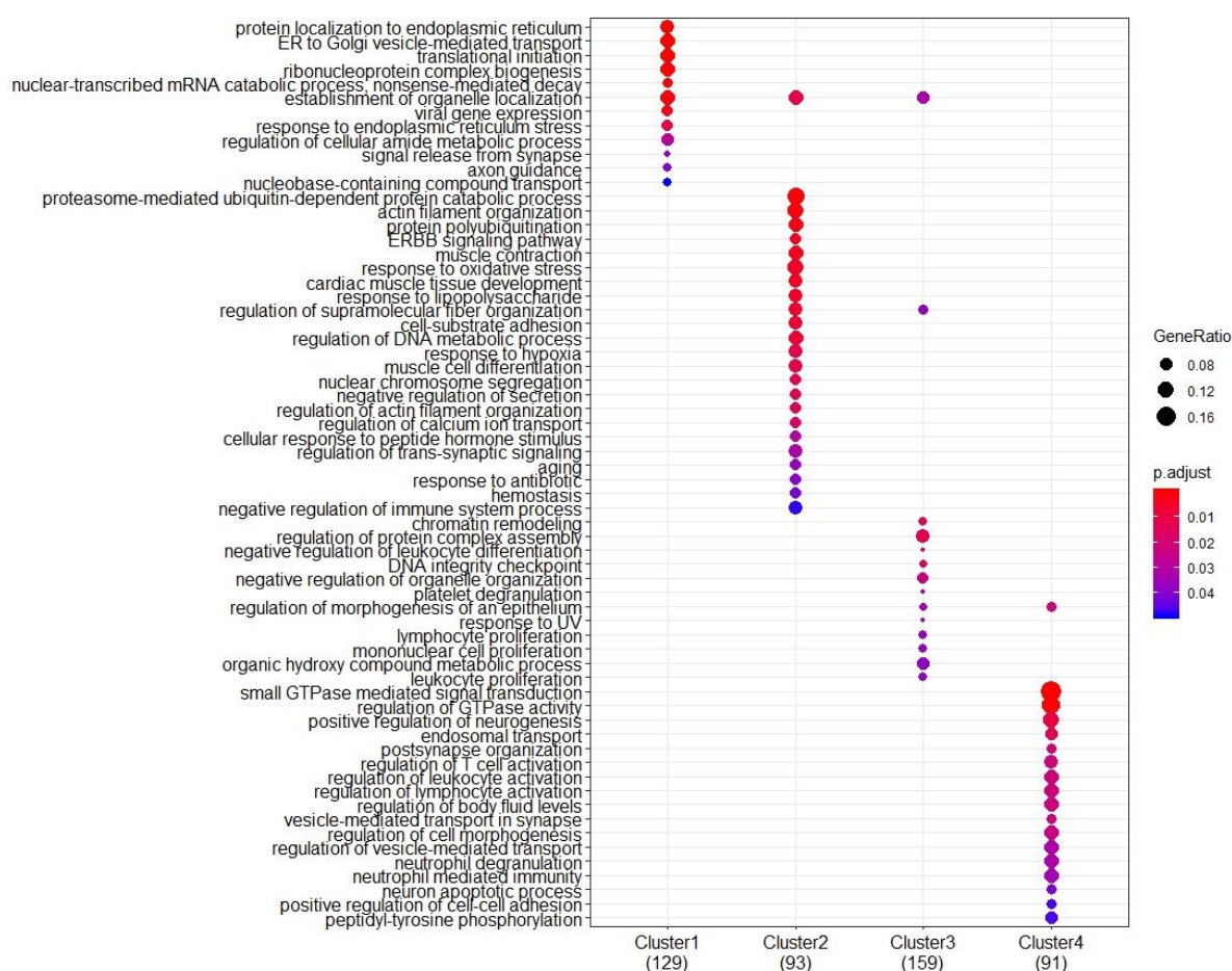
Fig. 4 Comparison between enriched pathways for each of the main modules identified. Interestingly, enriched pathways have little overlap among modules, indicating that they are functionally distinct.
