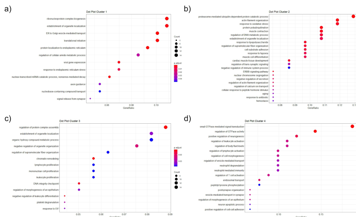
Fig. 3 Biological pathways enriched for differentially expressed genes in each of the functional modules identified by cluster analysis, namely, a) Cluster 1, b) Cluster 2, c) Cluster 3, and d) Cluster 4. Circle size represents the number of genes enriching for a given biological pathway and the color of the circle represents statistical significance, with red denoting higher statistical significance. GeneRatio is the ratio between the number of genes that have been enriched for a given pathway and the total number of genes that belong to the respective module.
