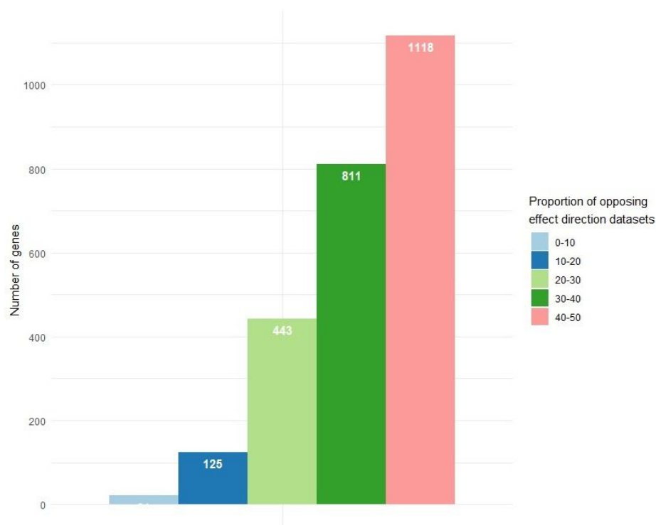
Fig. 1 Proportion (%) of datasets with divergent effect directions of differentially expressed genes identified in our meta-analysis. Only genes with opposite effect directions in a maximum of 30% of datasets containing information about them (i.e., genes included in the light blue, blue, and light green bars) were kept, totaling 589 genes.
