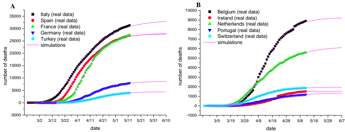
Figure 2. Fitting the cumulative COVID-19 deaths of each European country to the Richards function
