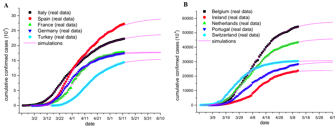
Figure 1. Fitting the cumulative confirmed COVID-19 cases of each European country to the Richards function
