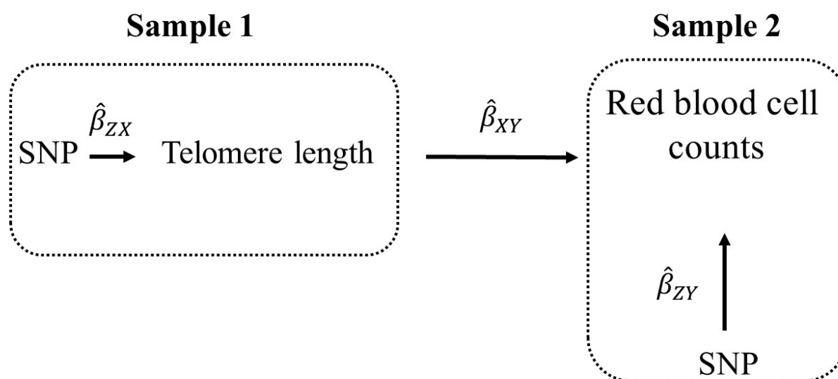
Fig. 1. Illustration of two-sample MR using the test of the causal effect of telomere length on red blood cell (RBC) counts as an example. Estimates of the SNP-telomere length associations ( \hat{\beta}_{ZX} )
