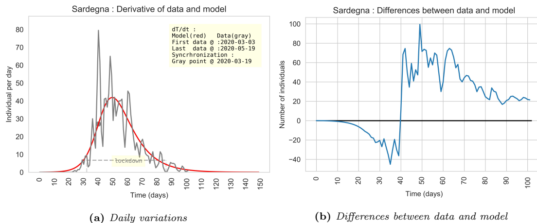
Figure 17: (a) Daily variation of T_{data} and of the T model (red). (b) Differences between T_{data} and the model T .
