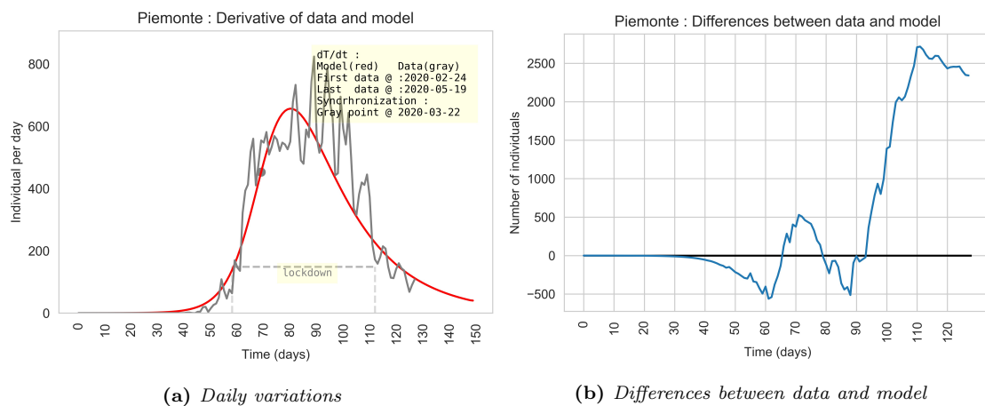
Figure 7: (a) Daily variation of T_{data} and of the T model (red). (b) Differences between T_{data} and the model T .
