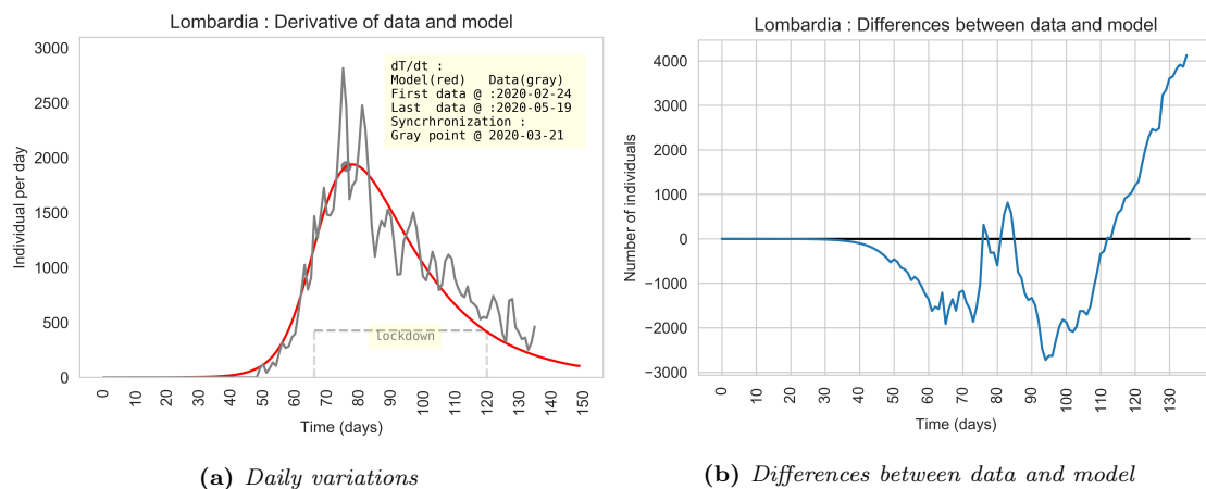
Figure 5: (a) Daily variation of T_{data} and of the T model (red). (b) Differences between T_{data} and the model T .
