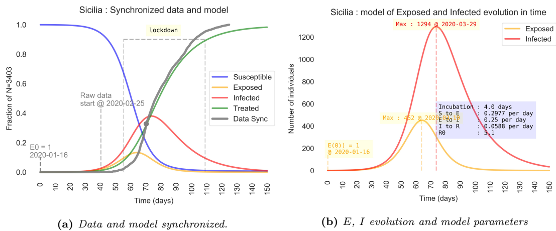
Figure 14: (a) The curve T of the model and T_{data} data has been synchronized at the point where the growth rate has been estimated. The ordinate scale is the ratio on the total number of cases N . (b) Detail of time evolution of E and I curves. The ordinate scale is the the number of individuals in the compartments E, I .
