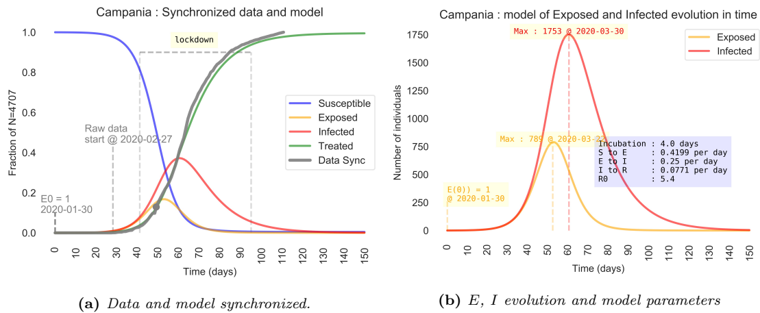
Figure 10: (a) The curve T of the model and T_{data} data has been synchronized at the point where the growth rate has been estimated. The ordinate scale is the ratio on the total number of cases N . (b) Detail of time evolution of E and I curves. The ordinate scale is the the number of individuals in the compartments E, I .
