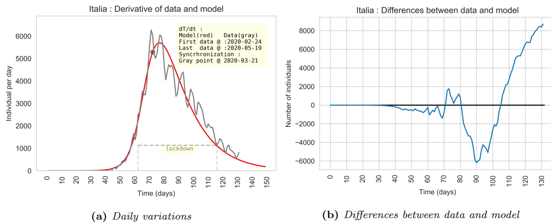
Figure 3: (a) Daily variation of T_{data} and of the T model (red). (b) Differences between T_{data} and the model T .
