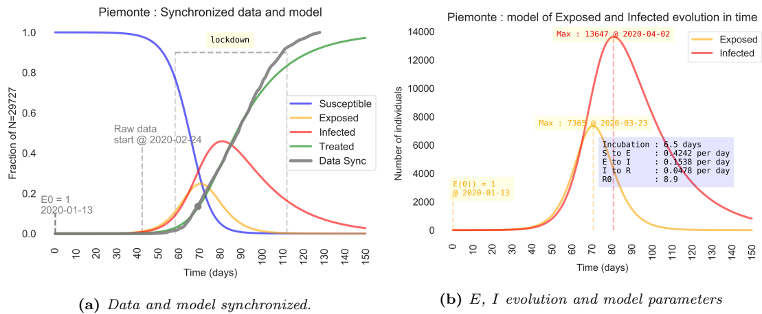
Figure 6: (a) The curve T of the model and T_{data} data has been synchronized at the point where the growth rate has been estimated. The ordinate scale is the ratio on the total number of cases N . (b) Detail of time evolution of E and I curves. The ordinate scale is the the number of individuals in the compartments E, I .
