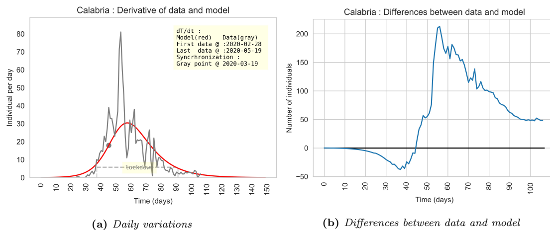
Figure 13: (a) Daily variation of T_{data} and of the T model (red). (b) Differences between T_{data} and the model T .
