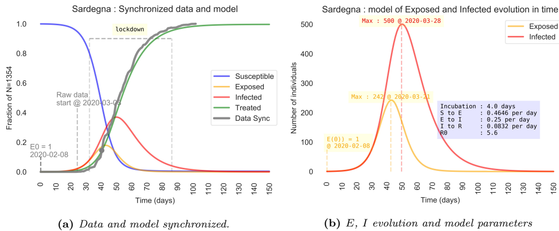
Figure 16: (a) The curve T of the model and T_{data} data has been synchronized at the point where the growth rate has been estimated. The ordinate scale is the ratio on the total number of cases N . (b) Detail of time evolution of E and I curves. The ordinate scale is the the number of individuals in the compartments E, I .
