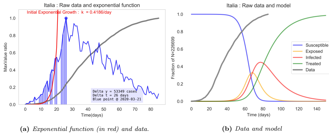
Figure 1: (a) Exponential function (red) used to approximate the data in the initial phase and daily variations of T_{data} (blue). (b) Response of the model to the perturbation eq. (15) near the DFE. The ordinate scales indicate in (a) the ratio with respect to the maximum values and in (b) the ratio on the total cases N of the number of individuals in the compartments E, I, S, T . In gray ( T_{data} ) are plotted the values of the COVID-19 cases detected in Italy until may 19th 2020: [1].
