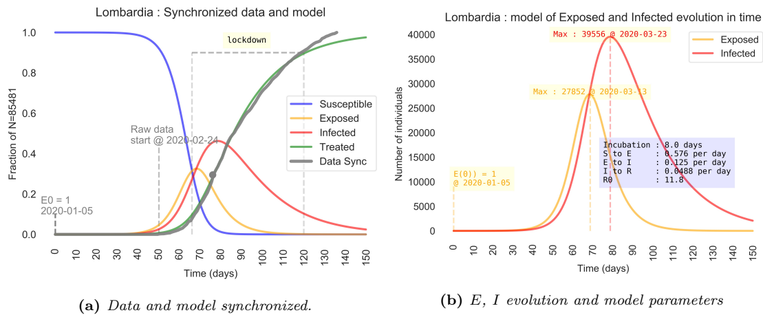
Figure 4: (a) The curve T of the model and T_{data} data has been synchronized at the point where the growth rate has been estimated. The ordinate scale is the ratio on the total number of cases N . (b) Detail of time evolution of E and I curves. The ordinate scale is the the number of individuals in the compartments E, I .
