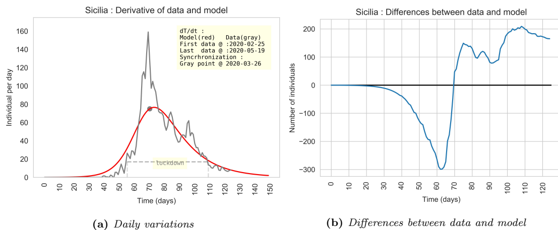
Figure 15: (a) Daily variation of T_{data} and of the T model (red). (b) Differences between T_{data} and the model T .
