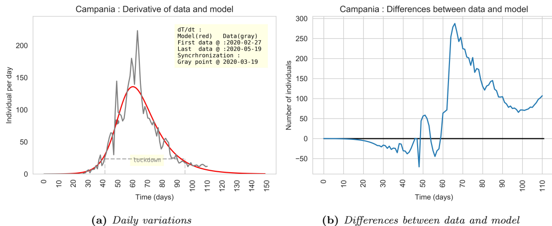
Figure 11: (a) Daily variation of T_{data} and of the T model (red). (b) Differences between T_{data} and the model T .
