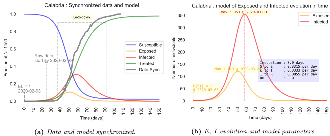
Figure 12: (a) The curve T of the model and T_{data} data has been synchronized at the point where the growth rate has been estimated. The ordinate scale is the ratio on the total number of cases N . (b) Detail of time evolution of E and I curves. The ordinate scale is the the number of individuals in the compartments E, I .
