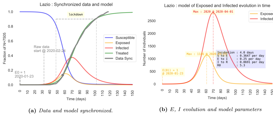
Figure 8: (a) The curve T of the model and T_{data} data has been synchronized at the point where the growth rate has been estimated. The ordinate scale is the ratio on the total number of cases N . (b) Detail of time evolution of E and I curves. The ordinate scale is the the number of individuals in the compartments E, I .
