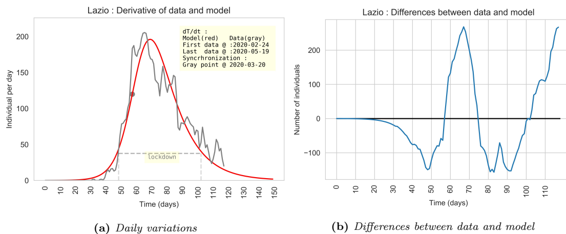
Figure 9: (a) Daily variation of T_{data} and of the T model (red). (b) Differences between T_{data} and the model T .
