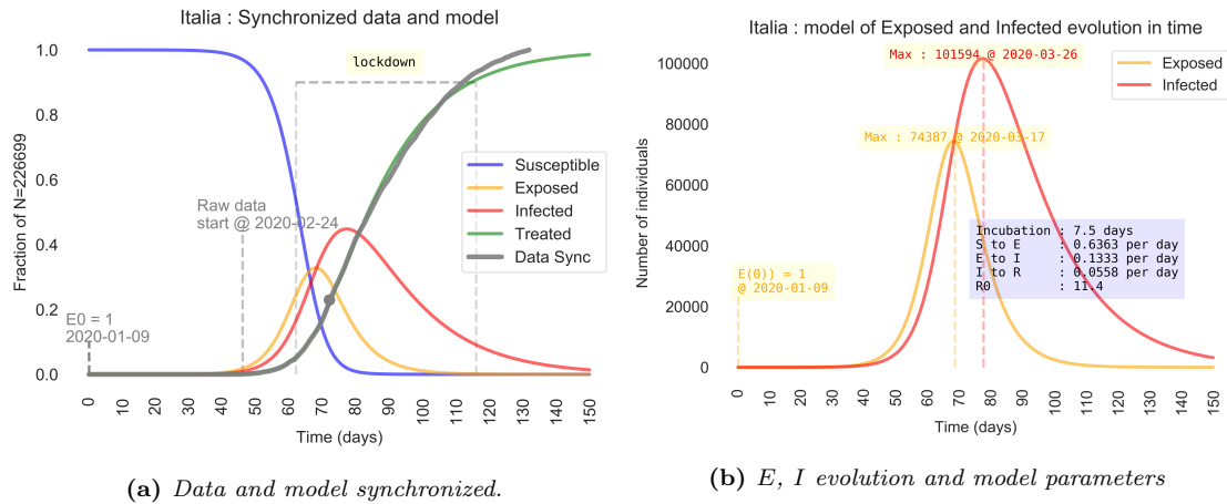
Figure 2: (a) The curves of model ( T ) and data ( T_{data} ) have been synchronized to the point where k is calculated (the grey point). The ordinate scale is the ratio on the total number of cases N . (b) Detail of time evolution of E and I curves. The ordinate scale is the the number of individuals in the compartments E, I .
