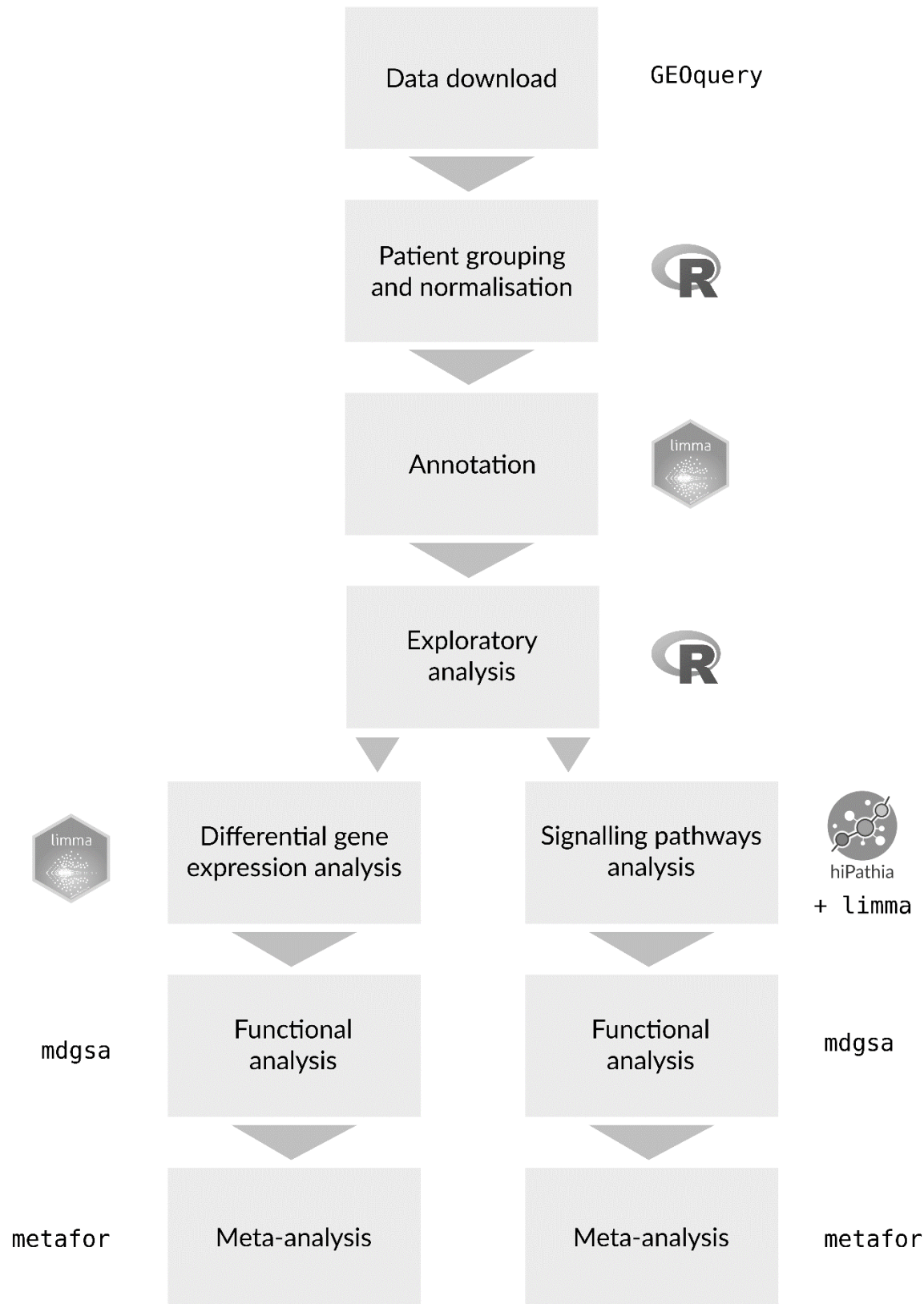
Fig. 1. Data-analysis workflow.
