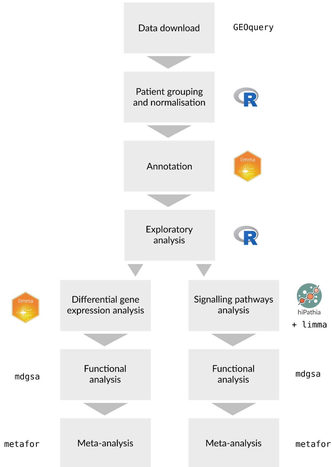
Fig. 4. Data-analysis workflow.
