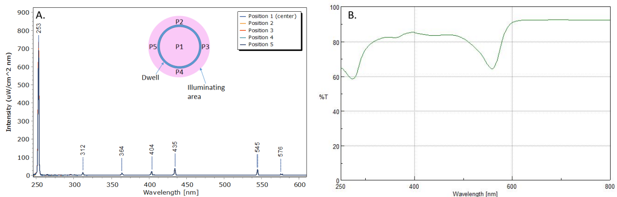
Figure 5. Mercury lamp spectrum measured in the five positions (Panel A). Inset: scheme of the illuminated dwell and the measuring position. UV-vis transmission spectrum of the Dulbecco's Modified Eagle's Medium (DMEM) in a 1 mm quartz cuvette (Panel B).
