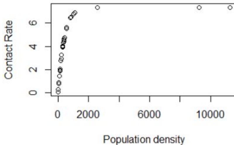
Supplementary Figure3: State-wise population density versus contact rate simulation.
