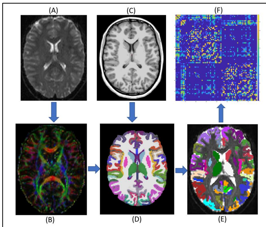
Figure 1. Individual level imaging data analysis and network construction. (A) DTI data; (B) Estimated tensor directions with 2-crossing fiber model; (C) T1-weighted structural MRI data; (D) Parcellated structural image based on Desikan-Killiany Atlas; (E) Seed masks in diffusion space, which binarized and transformed from structural space; (F) Symmetric and weighted 78 \times 78 connectivity matrix. The edges were calculated based on the number of fibers in tractography. DTI: Diffusion Tensor Imaging.
