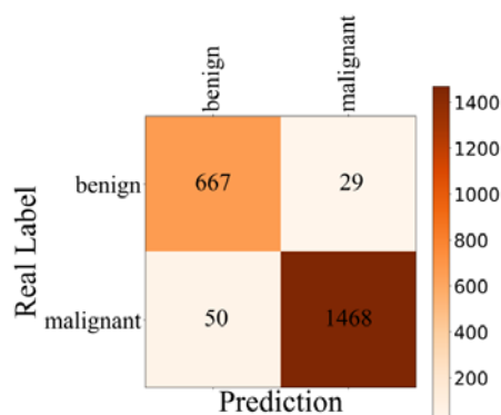
Figure 2. confusion matrix
