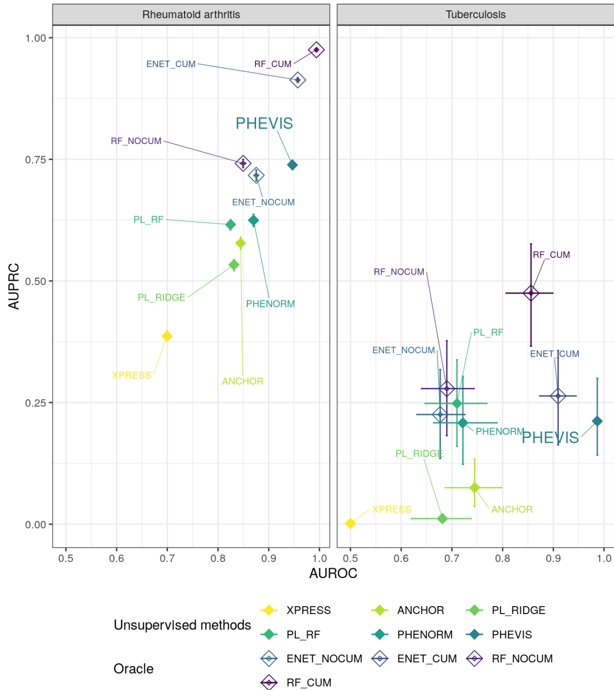
Figure 2: Phenotyping unsupervised and supervised methods comparison. University Hospital of Bordeaux. Confidence Intervals for AUROC and AUPRC are represented by horizontal and vertical segments respectively. PL_RIDGE: POLAR method with ridge logistic regression. PL_RF: POLAR method with random forest. ENET: Supervised elastic-net logistic regression with (CUM) or without (NOCUM) cumulated variables. RF: Supervised random forest with or without cumulated variables.
