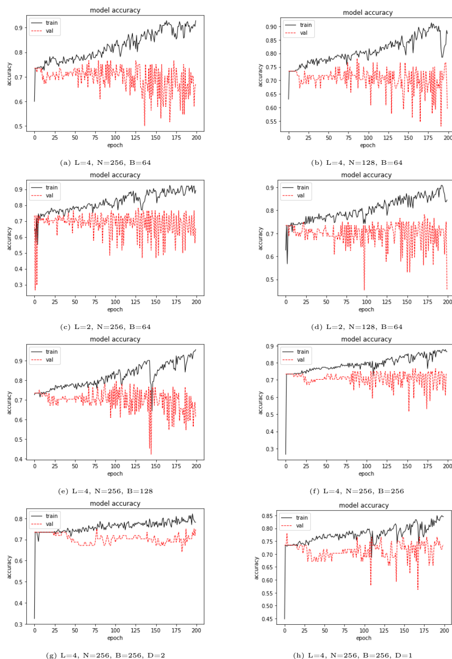
Fig.5: Ablation Study: Performance of the network on varying batch size, number of layers and number of neurons for predicting hypertension. Figure 5 (h) one dropout layer is included and the in Figure 5 (g) two dropout layers are included in the model.
