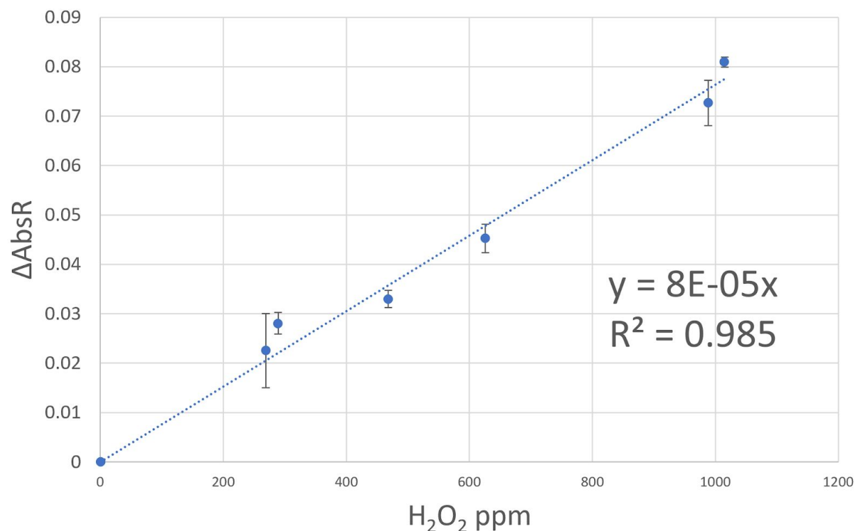
Fig. 2. Calibration curve for H_2O_2 solutions 0-5%. Error bars represent the standard deviation of the red light component absorbance.
