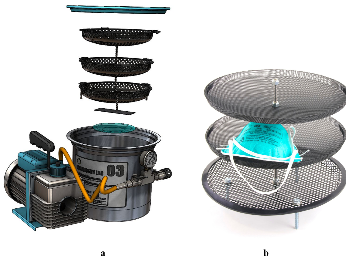
Fig. 5. a. A digital rendering of the vacuum pump and vacuum chamber with glass lid, hydrogen peroxide dish, and mask loader tray. b. A photograph of a mask loader tray that can fit up to 12 N95 respirators, consisting of three
