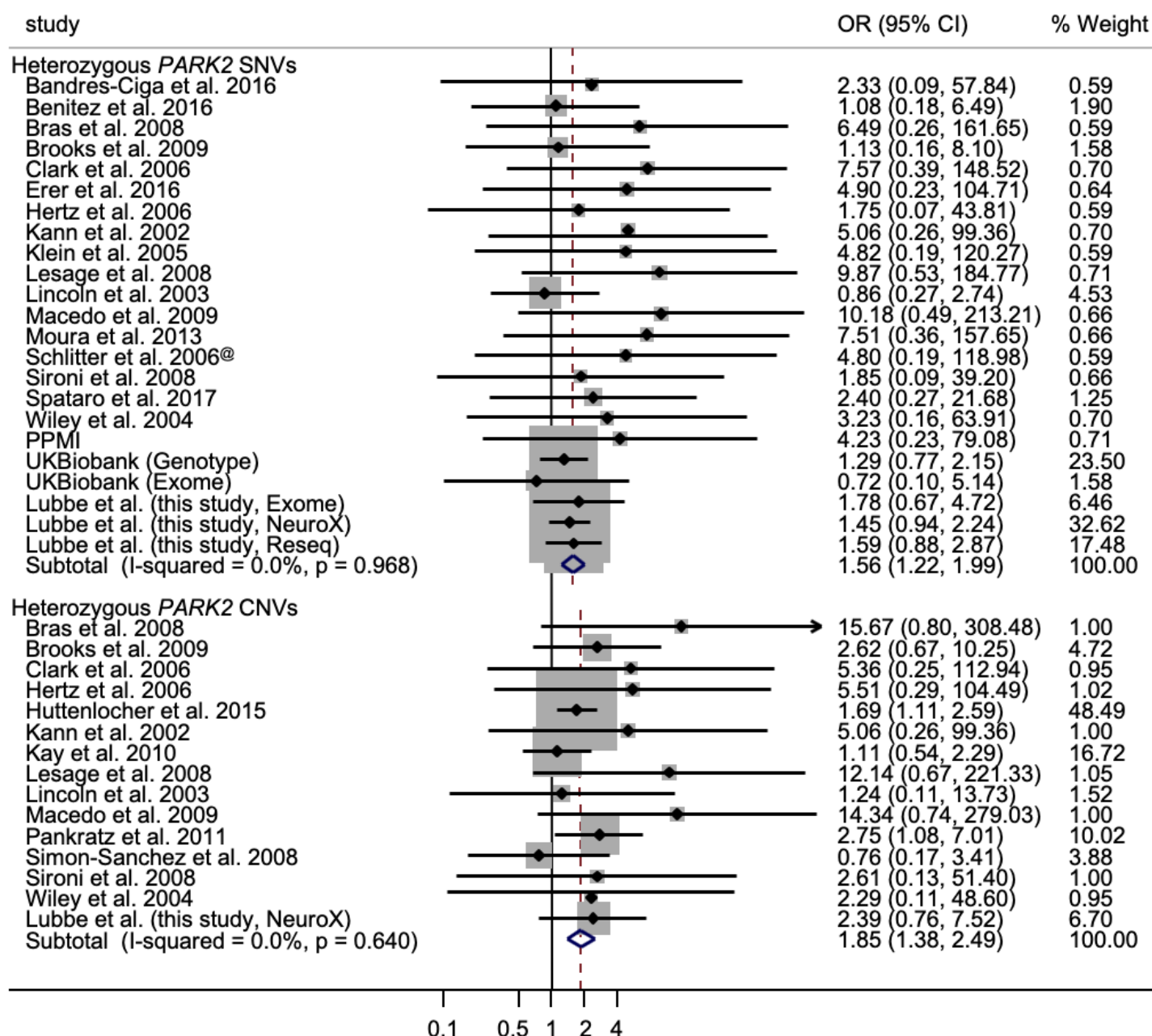
Figure 3: Forest plot of the odds ratio (OR) of the Parkinson's risk associated with heterozygous PARK2 single nucleotide variant (SNV) and copy number variant (CNV) carriers.
