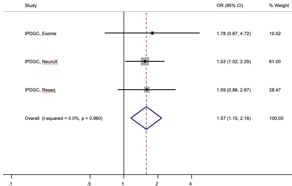
Figure 1: Forest plot of the odds ratio (OR) of the Parkinson's risk associated with heterozygous PARK2 mutations in three independent International Parkinson's disease Genomics Consortium (IPDGC) cohorts.
