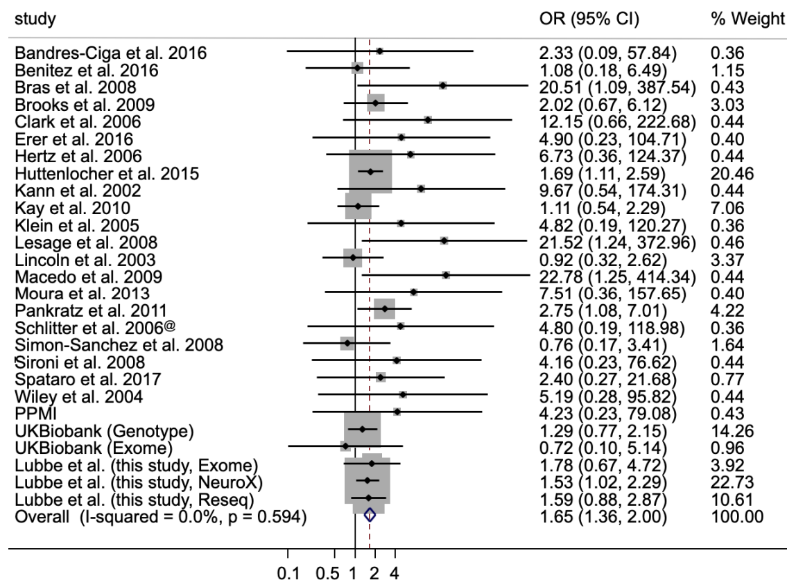
Figure 2: Forest plot of the odds ratio (OR) of the Parkinson's risk associated with heterozygous PARK2 mutations.
