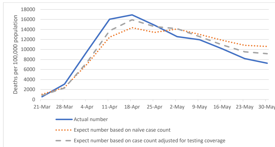
Figure 1. Actual and expected number of weekly US COVID-19 deaths
