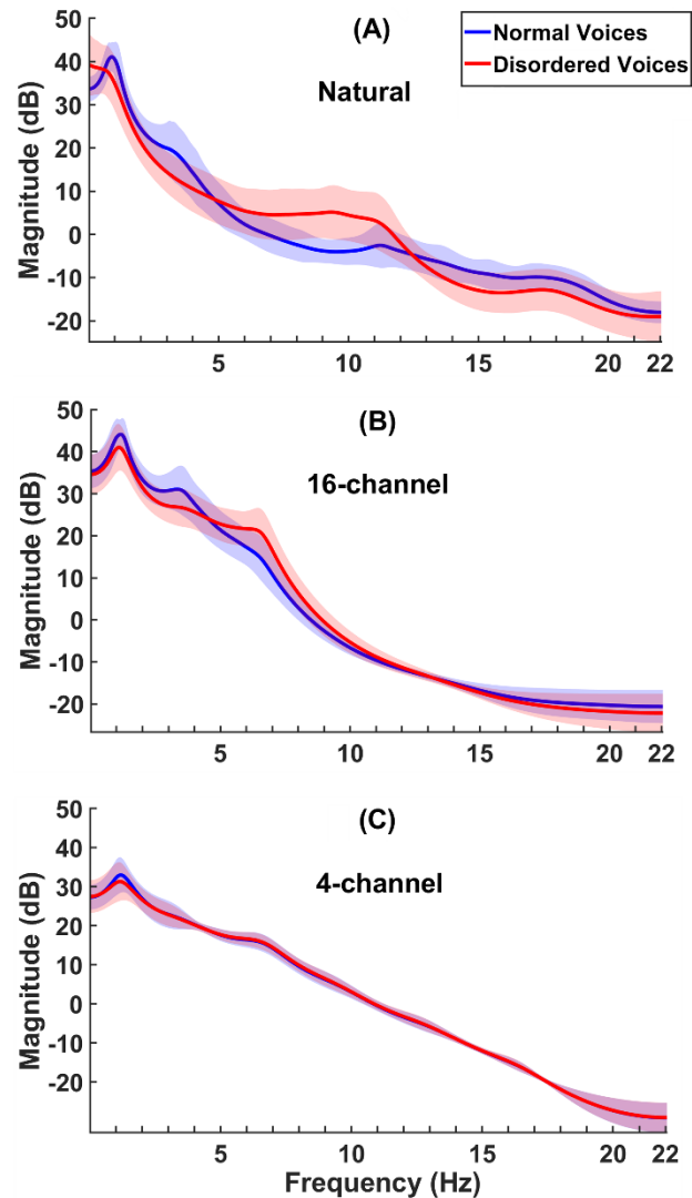
359 Fig. 2. (Color online) Average magnitude spectra of voice stimuli with normal (blue or dark gray 360 lines) and disordered (red or light gray lines) qualities for (A) unprocessed voices, (B) simulated 361 cochlear-implant voices with 16-channel, and (C) 4-channel in the CI noise-vocoder. The standard 362 deviations of the magnitude spectra are also shown as the blue (dark gray) shaded area across the 363 average blue line (dark gray) for the group of normal voices and as the red (light gray) shaded area 364 across the average red line (light gray) for the group of disordered voices.
