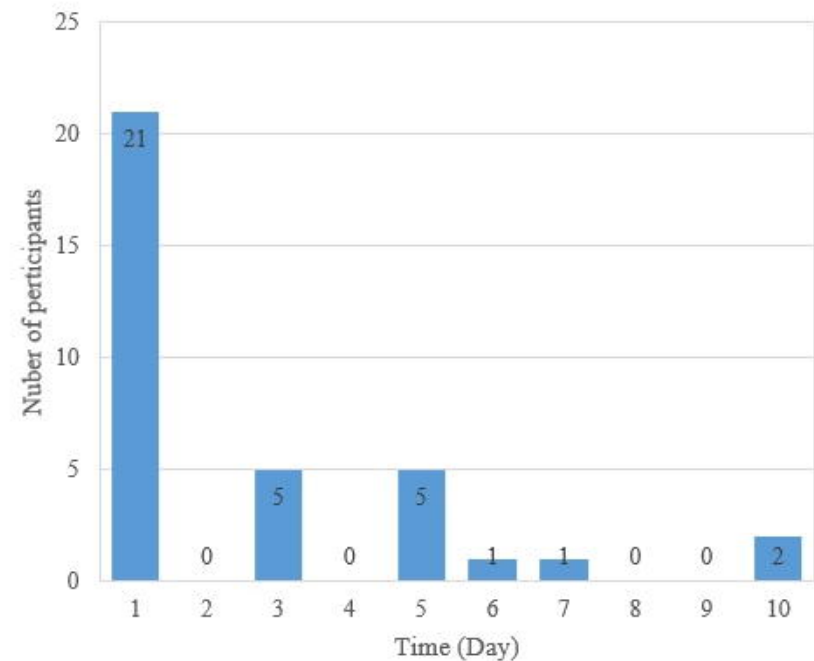
New daily cases of non-adherence
