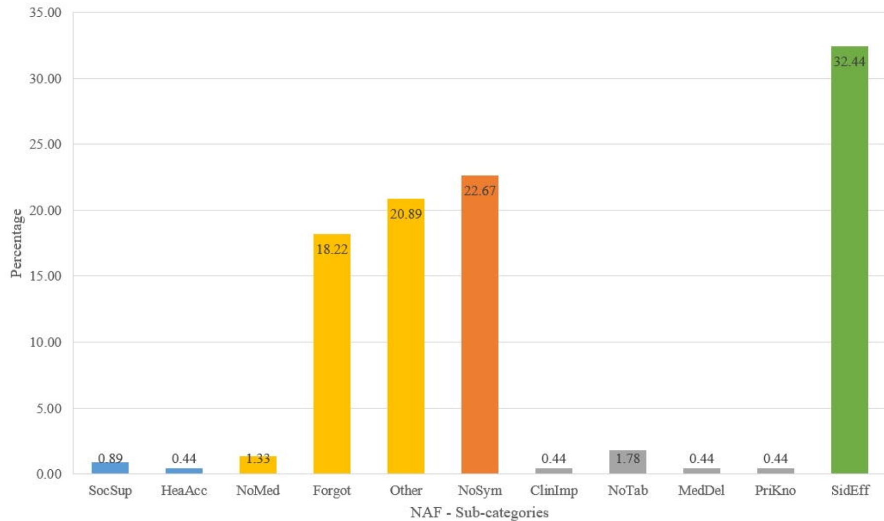
Contribution to P(NA) - All NAFs
