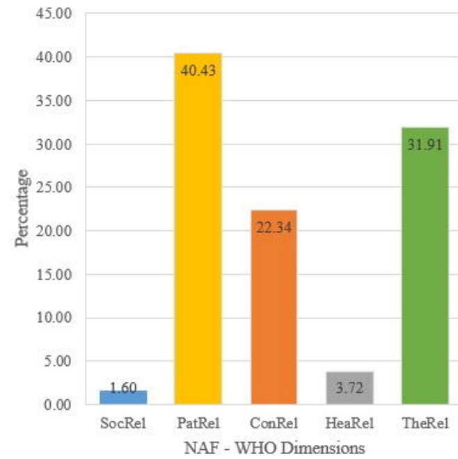
Contribution to P(NA) - Dimensions
