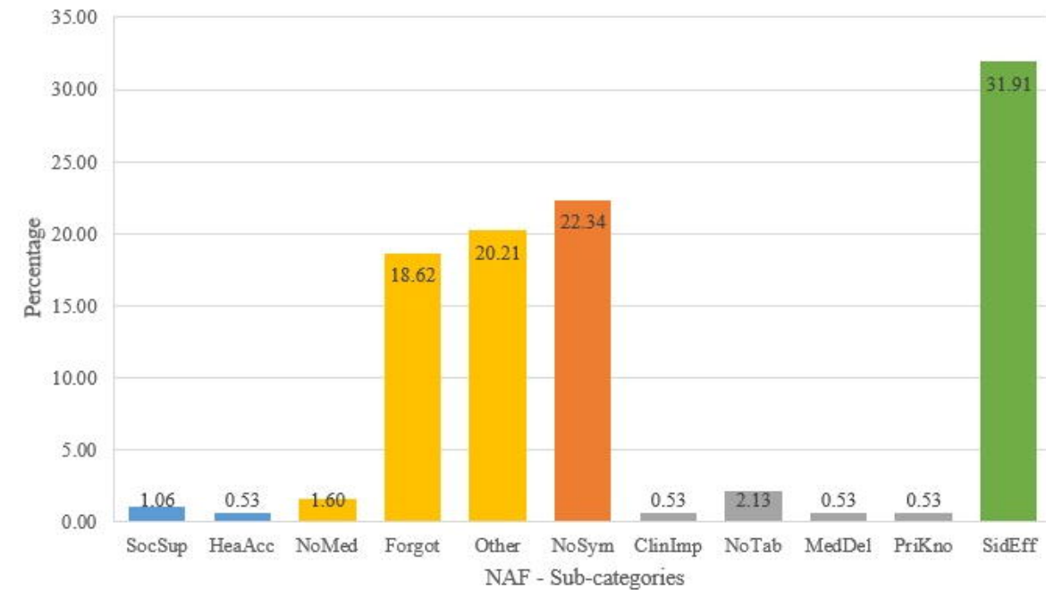
Contribution to P(NA) - All NAFs
