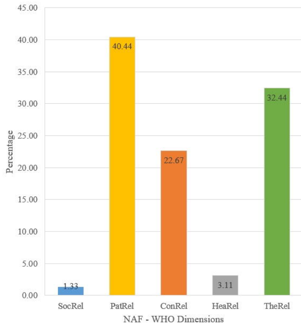
Contribution to P(NA) - Dimensions
