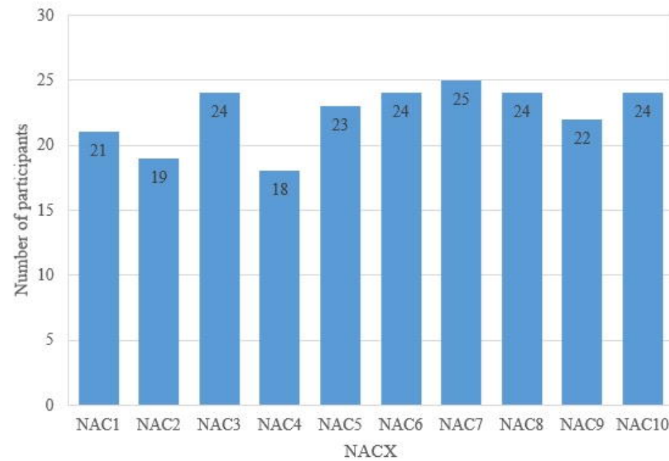
Non-adherent count (NAC)
