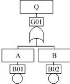
Y: OR Gate
