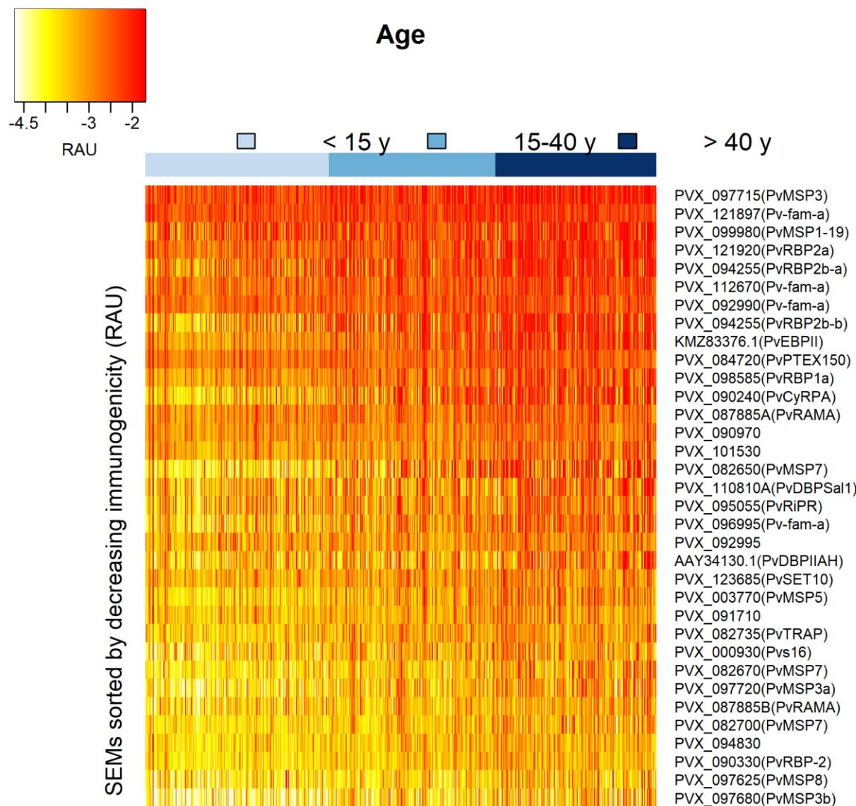
Fig 2. Heatmap of antibody responses to P. vivax serological exposure markers in the Peruvian cohort. Relative antibody units (RAU) were log10 transformed.
