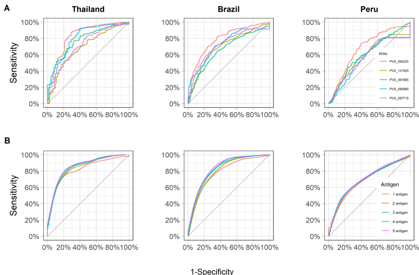
Fig 4. Diagnostic performance for classifying recent exposure using antibody responses. (A) Receiver operating characteristic (ROC) curve displays the diagnostic performance of 5 top antibody responses individually: PVX_094255 (PvRBP2b), PVX_121920 (PvRBP2a), PVX_087885 (PvRAMA), PVX_099980 (PvMSP1 19 ) and PVX_097715 (hypothetical PvMSP3) in the study sites. (B) ROC curves displaying the diagnostic performance to detect recent infections given by combinations of the top 5 antibody responses.
