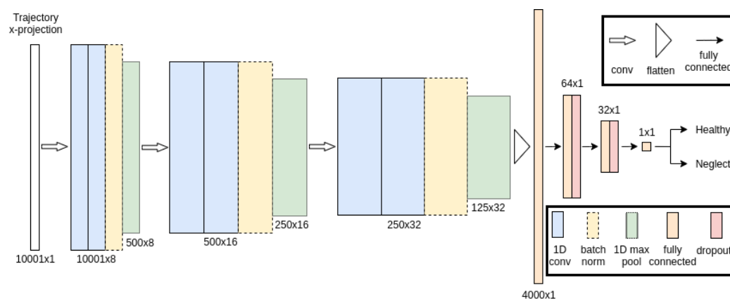
Figure 2: (Left). The CNN architecture used in our experiments. Three convolutional blocks with batch normalization and pooling are followed by two dense layers with dropout. Dimensions of each layer are reported in the image. The final output is the probability that each input trajectory has to either belonging to a healthy control or to a patient with spatial neglect. To assign the final class (healthy vs. neglect) to one subject, we performed a majority voting across all trajectories of that subject.
