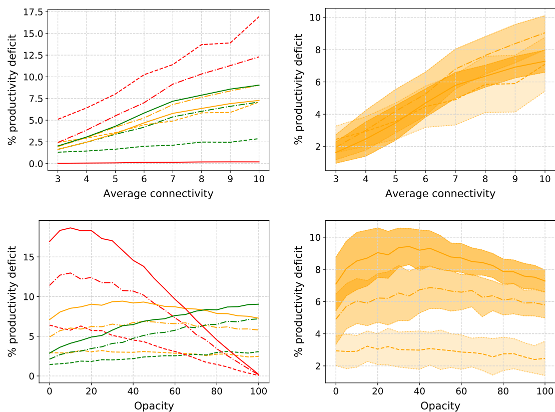
Figure 10: Same as Fig. 6 but for running hot
