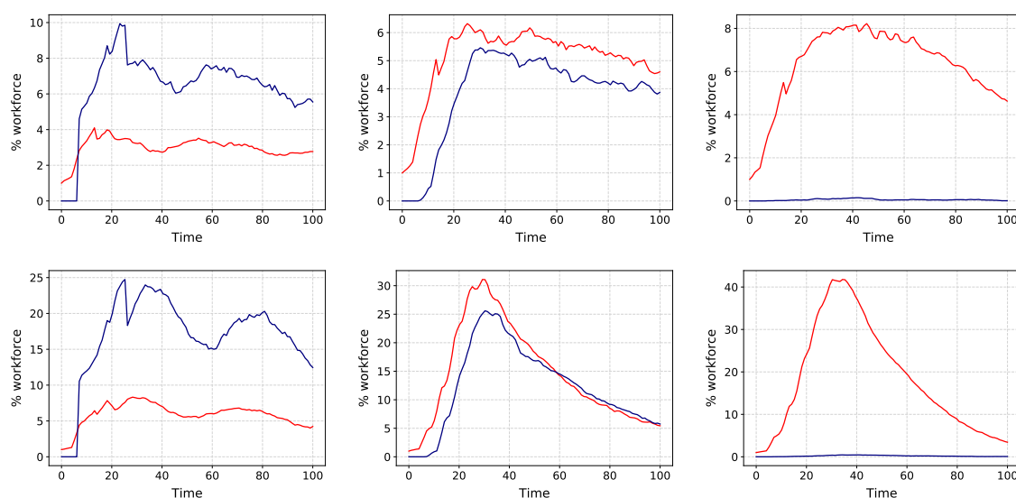
Figure 7: Same as Fig. 3 but in the case of hot runs.
