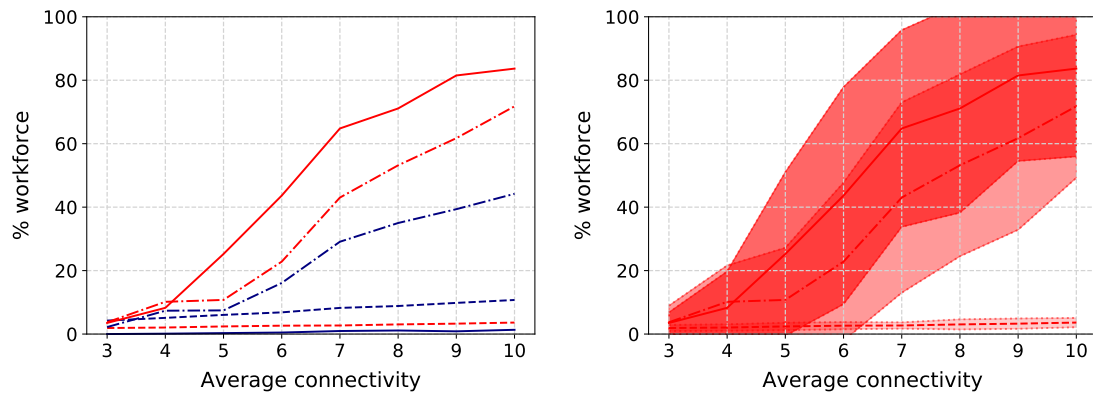
Figure 4: (Left) Proportion of workforce that become unwell at least once (red lines) or go home (blue lines) as a function of the average contact network size d . Results are shown for three different opacities O = 0\% (dashed lines), O = 50\% (dot-dashed) and O = 100\% (solid). (Right) Mean, plus and minus one standard deviation of the becoming ill proportions.
