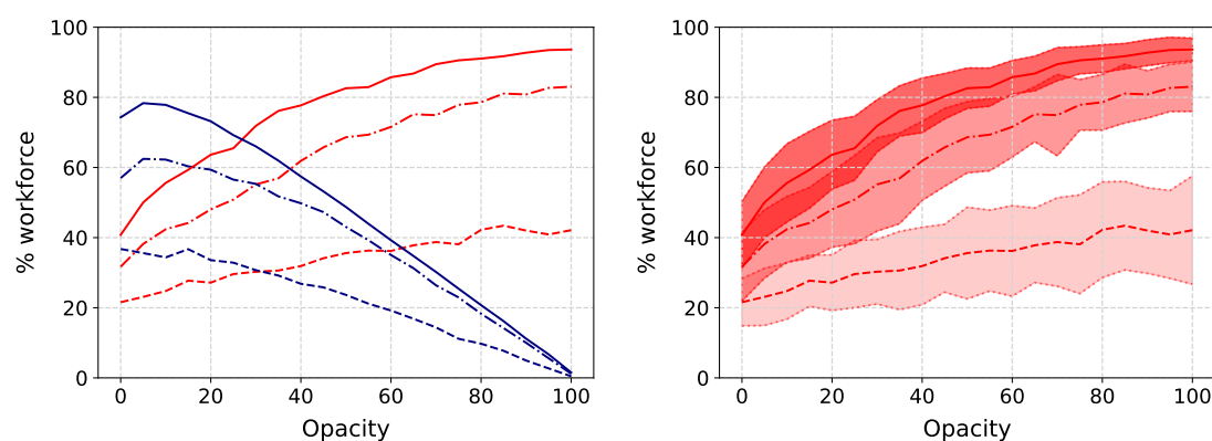
Figure 9: Similar to Fig. 5 but for running hot.
