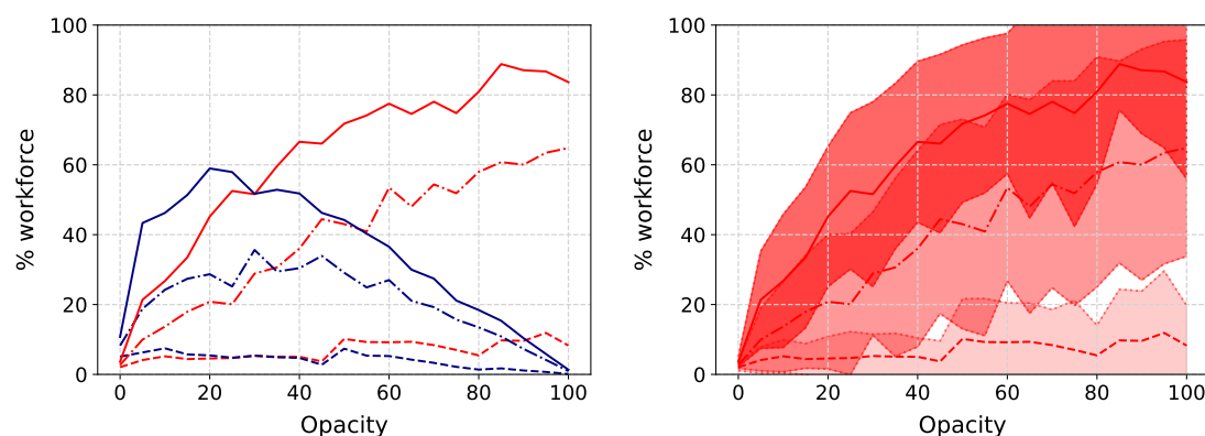
Figure 5: Similar to Fig. 4 but showing variation with opacity for three different values of average degree; d = 4 (dashed lines), d = 7 (dot-dashed) and d = 10 (solid).
