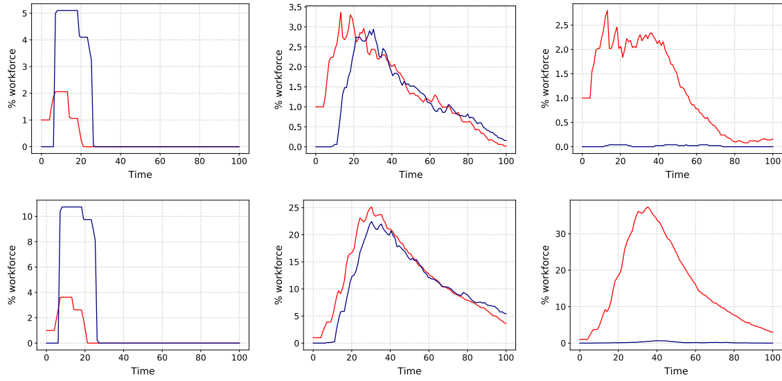
Figure 3: Examples of cold runs for different size of contact network d and degree of opacity O against time. In each plot, the red curve gives the proportion of unwell individuals (in state U ) and the blue curve gives the proportion who are at home (with p_i = 0 ). Parameter values are: (top left) d = 4 , O = 0 ; (top middle) d = 4 , O = 50\% ; (top right) d = 4 , O = 100\% ; (bottom left) d = 10 , O = 0 ; (bottom middle) d = 10 , O = 50\% ; (bottom right) d = 10 , O = 100\% .
