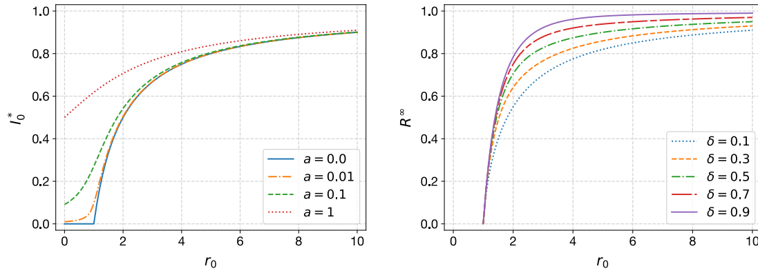
Figure 11: (Left) Plot of I_0^* given by (14) against r_0 for different a \geq 0 in the case of no immunity ( \delta = 0 ). (Right) Positive value of R^\infty obtained by solving (15) for different values of \delta > 0 in the running cold case ( a = 0 ).
