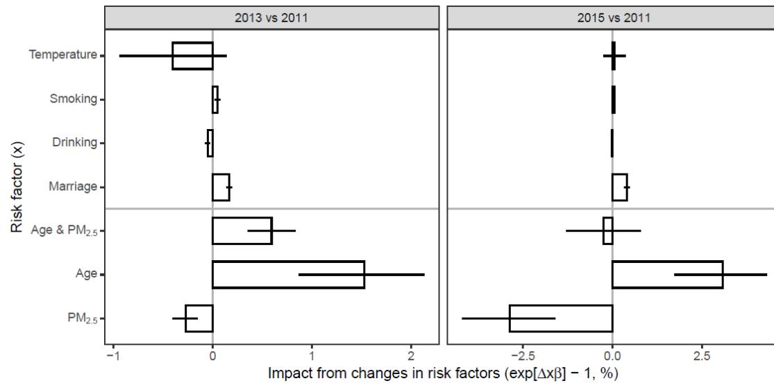
Figure 4. Impacts of reducing PM 2.5 concentration, aging, and changes in other factors on the CES-D-10 score. The changes in risk factors ( \Delta x ) were evaluated using a fixed group of subjects who participated in all three China Health and Retirement Longitudinal Study (CHARLS) waves; the corresponding coefficients were estimated from the longitudinal model with standard adjustment (Figure 2) and presented in Table S3; for each variable, the value in 2011 was acted the reference to evaluate the impact attributable to its temporal changes.
