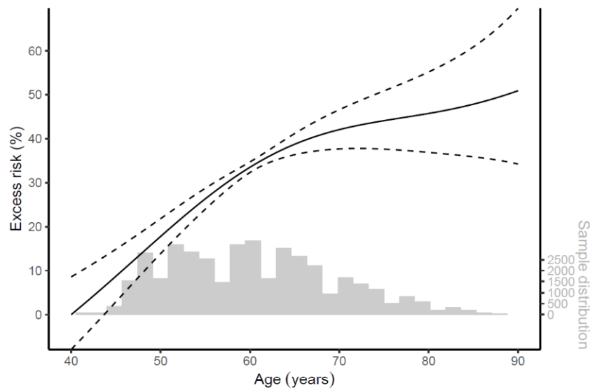
Figure 3. Nonlinear effects of (a) PM_{2.5} concentration and (b) age on the CES-D-10 score. Dashed lines, pointwise 95% confidence intervals. The histograms show the distribution of PM_{2.5} exposure and age.
