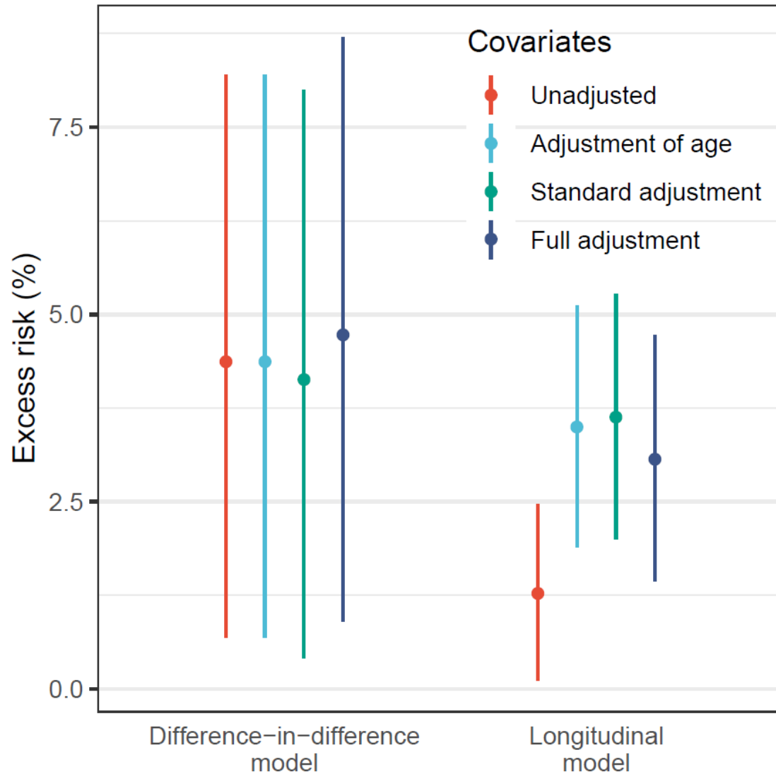
Figure 2. Estimated associations between the depression score and PM_{2.5} concentration. In the difference-in-difference (DID) analysis, the model adjusted for age incorporated age at 2011 as a covariate; the standard adjustment also involved the fixed variables of urban/rural residence, sex, and education, as well as the longitudinal variables of ambient temperature, marriage status, smoking, and drinking. The full adjustment also considered longitudinal changes in cooking energy type, building type, residential rent payment, presence of an in-house telephone, and indoor temperature maintenance. The longitudinal models adjusted for the constant variables in a similar manner as in the DID models; however, adjustment of the longitudinal variables was based on the values recorded in each survey wave, rather than their between-wave changes therein.
