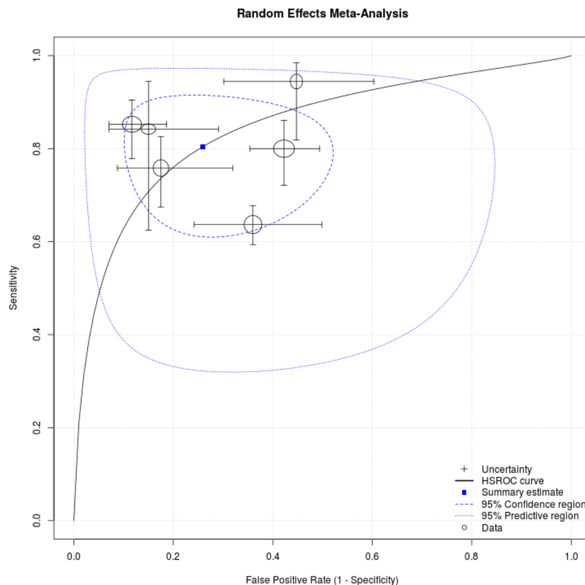
391 Figure 3: ROC plot displaying extrapolated SROC curve, the summary estimate for sensitivity and 392 specificity, and percentage study weights
