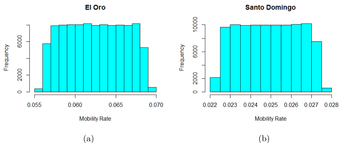
Figure 10: Histogram plot for the mobility rate of El Oro (a) and Santo Domingo (b) provinces, generated from the equation ?? by varying the number of inter-provincial buses available in each province and the number of people such buses transport in a day.
