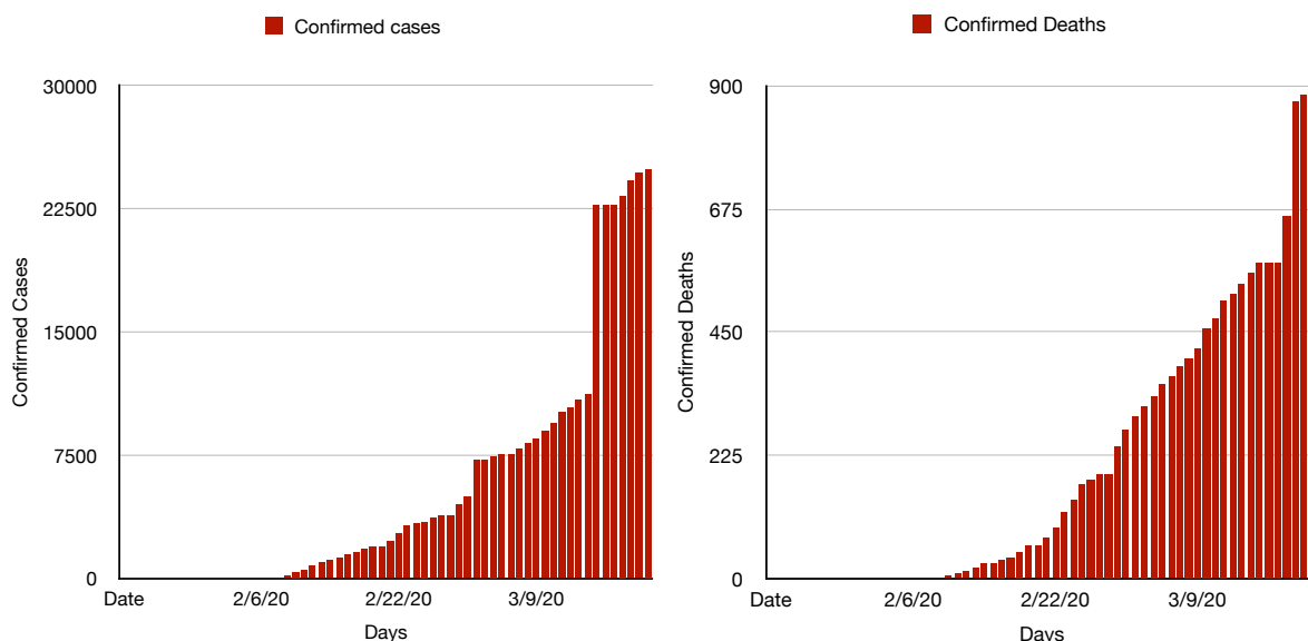
Figure 8: Evolution of confirmed cases and deaths in Ecuador
