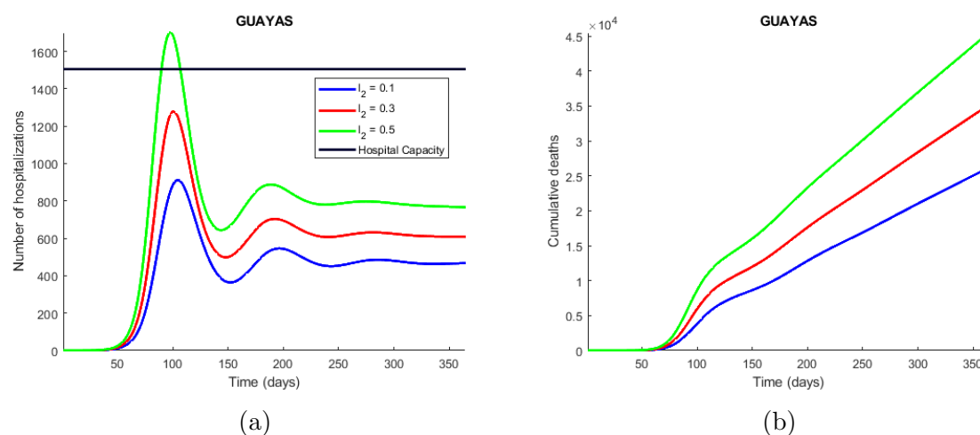
Figure 4: Time series plot of the number of hospitalizations (a), and cumulative deaths (b) predicted by the model. The simulations were done for Guayas province with the parameters values presented in Table 2 and varying the proportion of symptomatic infectious people that are not strictly isolated ( l_2 ) between 0.1 (10 % of the symptomatic infectious people are not strictly isolated) and 0.5. The legend specifies the values for the studied parameter that produce the corresponding curves, considering the explained meaning of such values. The horizontal line represents the hospitals capacity in the province.
