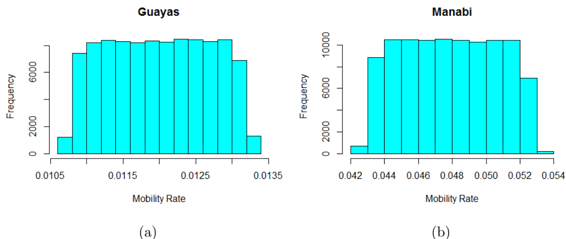
Figure 9: Histogram plot for the mobility rate of Guayas (a) and Manabi (b) provinces, generated from the equation ?? by varying the number of inter-provincial buses available in each province and the number of people such buses transport in a day.
