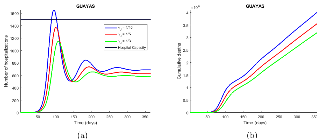
Figure 3: Time series plot of the number of hospitalizations (a), and cumulative deaths (b) predicted by the model. The simulations were done for Guayas province with the parameters values presented in Table 2 and varying the symptomatic infectious quarantine rate ( \gamma_J ) between 1/3 (people showing COVID-19 symptoms are sent into isolation within 3 days) and 1/10. The legend specifies the values for the quarantine rates that produce the corresponding curves, considering the explained meaning of such values. The horizontal line represents the hospitals capacity in the province.
