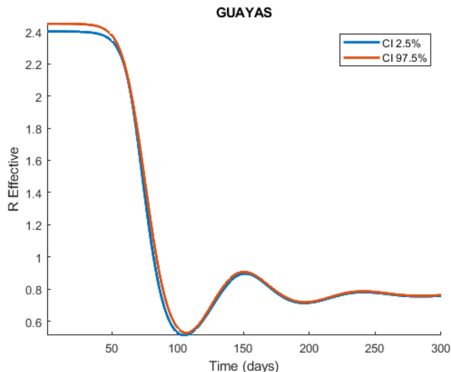
Figure 6: Time series plot of the effective reproduction number ( \mathcal{R}_e ) for the Guayas province. The curves represent the upper and lower bounds of the 95% confidence interval of \mathcal{R}_e . These simulations were made from the COVID-19 model presented in this study, using the parameter values from Table 2 and sampling the four unknown parameters.
