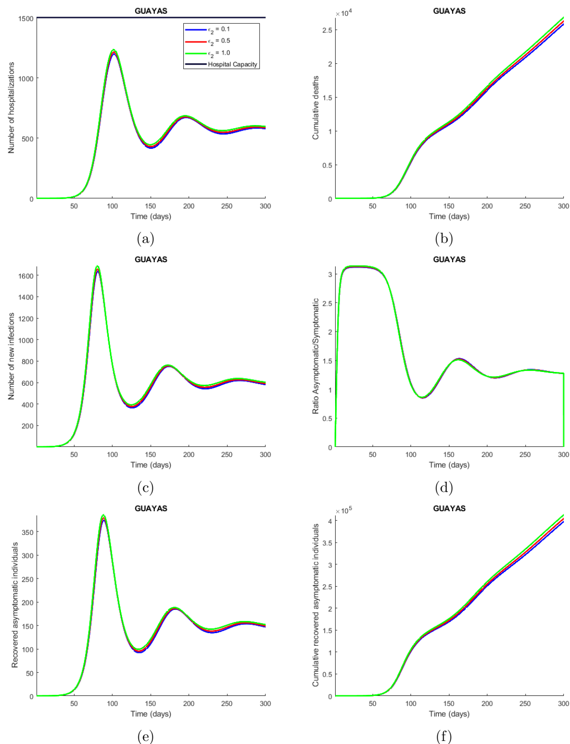
Figure 16: Time series plot of the number of hospitalizations (a), cumulative deaths (b), number of new infections (c), ratio asymptomatic/symptomatic (d), number of new recovered asymptomatic individuals (e) and cumulative recovered asymptomatic individuals (f) predicted by the model. These simulations were done for Guayas province with the parameters values presented in Table 2 and varying the infectiousness of hospitalized individuals ( \epsilon_2 ) between 0.1 (hospitalized individuals are only 10 % infectious as compared with those symptomatic individuals that have not been detected) and 1. The legend specifies the values for the studied parameter that produce the corresponding curves, considering the explained meaning of such values. The horizontal line represents the hospitals capacity in the province.
