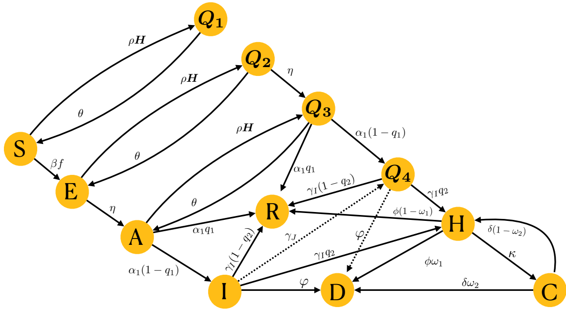
Figure 1: Schematic flow diagram for our model. The model consists of twelve sub populations and their definitions are given in Table 1.
