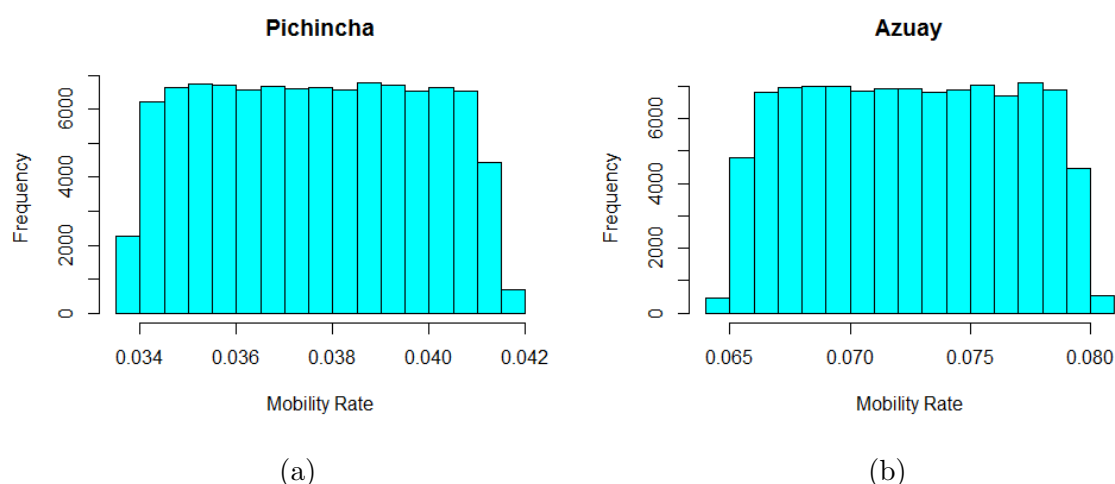
Figure 12: Histogram plot for the mobility rate of Pichincha (a) and Azuay (b) provinces, generated from the equation ?? by varying the number of inter-provincial buses available in each province and the number of people such buses transport in a day.
