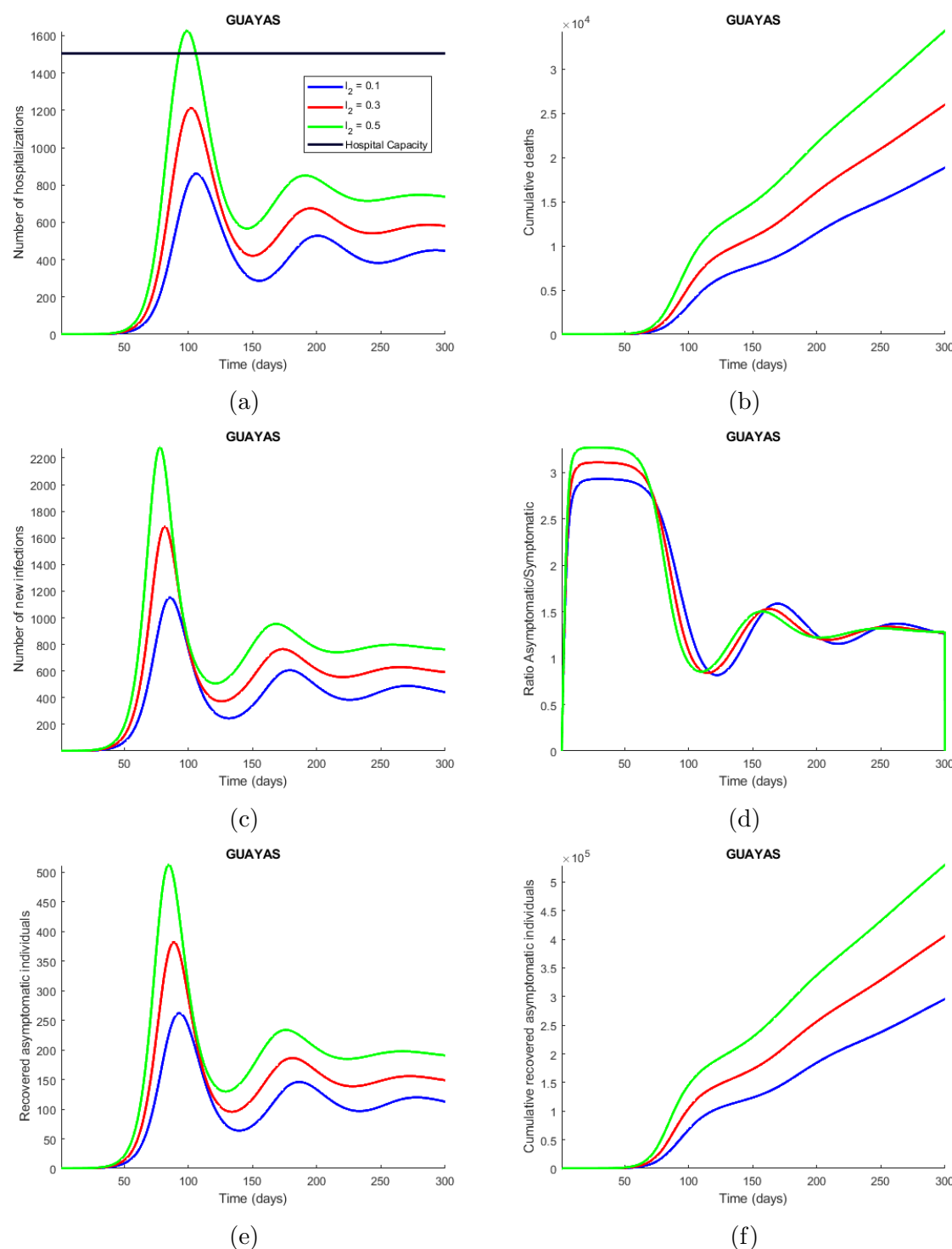
Figure 15: Time series plot of the number of hospitalizations (a), cumulative deaths (b), number of new infections (c), ratio asymptomatic/symptomatic (d), number of new recovered asymptomatic individuals (e) and cumulative recovered asymptomatic individuals (f) predicted by the model. These simulations were done for Guayas province with the parameters values presented in Table 2 and varying the proportion of symptomatic infectious people that are not strictly isolated ( l_2 ) between 0.1 (10 % of the symptomatic infectious people are not strictly isolated) and 0.5. The legend specifies the values for the studied parameter that produce the corresponding curves, considering the explained meaning of such values. The horizontal line represents the hospitals capacity in the province.
