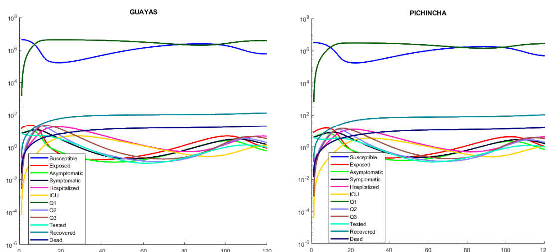
Figure 17: Simulation of the complete model without mobility (Model 2.2.2), considering limited number of ICU beds for two of the most affected provinces, for two of the most affected provinces
