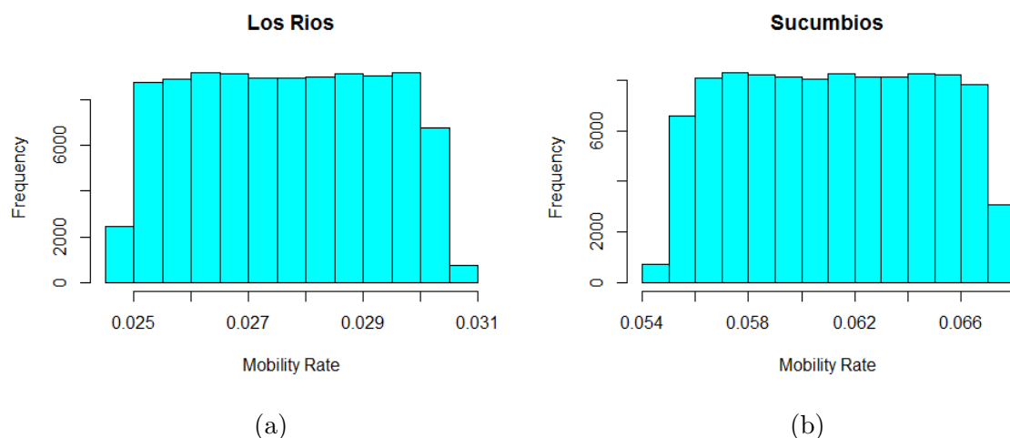
Figure 11: Histogram plot for the mobility rate of Lor Rios (a) and Sucumbios (b) provinces, generated from the equation ?? by varying the number of inter-provincial buses available in each province and the number of people such buses transport in a day.
