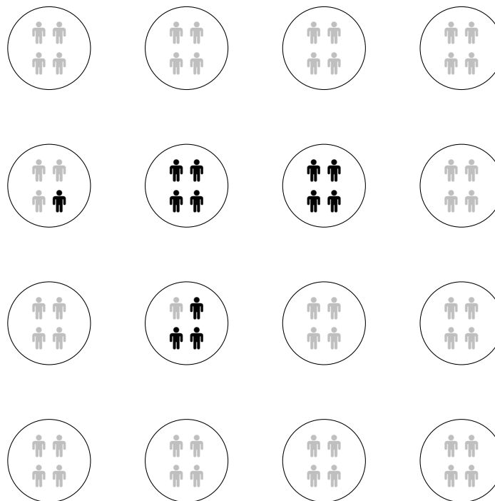
Figure 1. Household model. Black symbols correspond to infected individuals.
