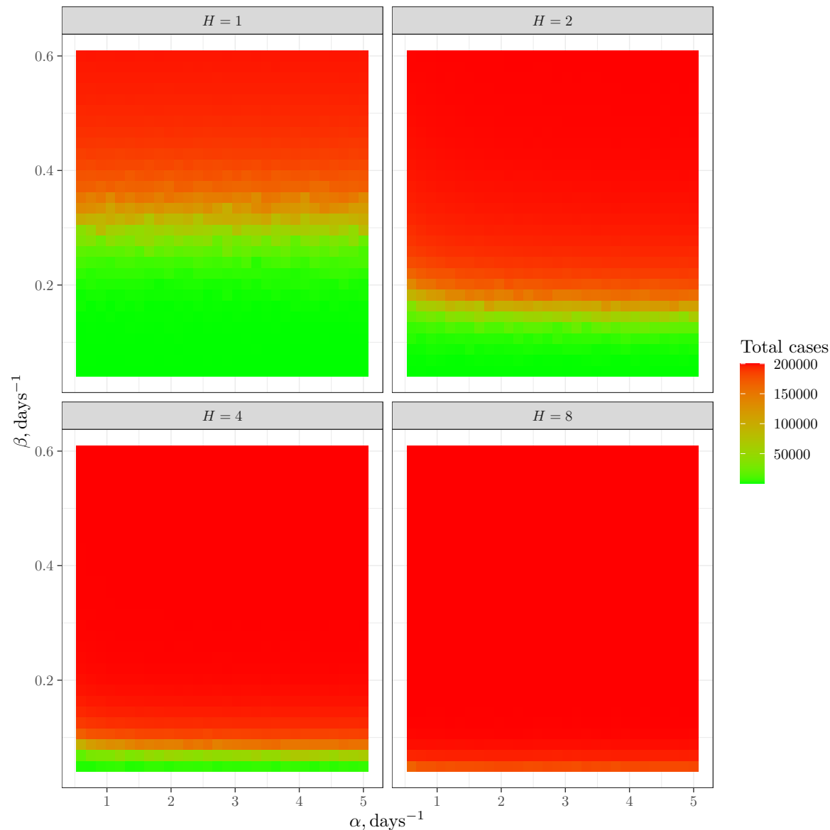
Figure 6. The total number of cases for simulations with N = 200\,000 . Each subfigure corresponds to a value of H .
