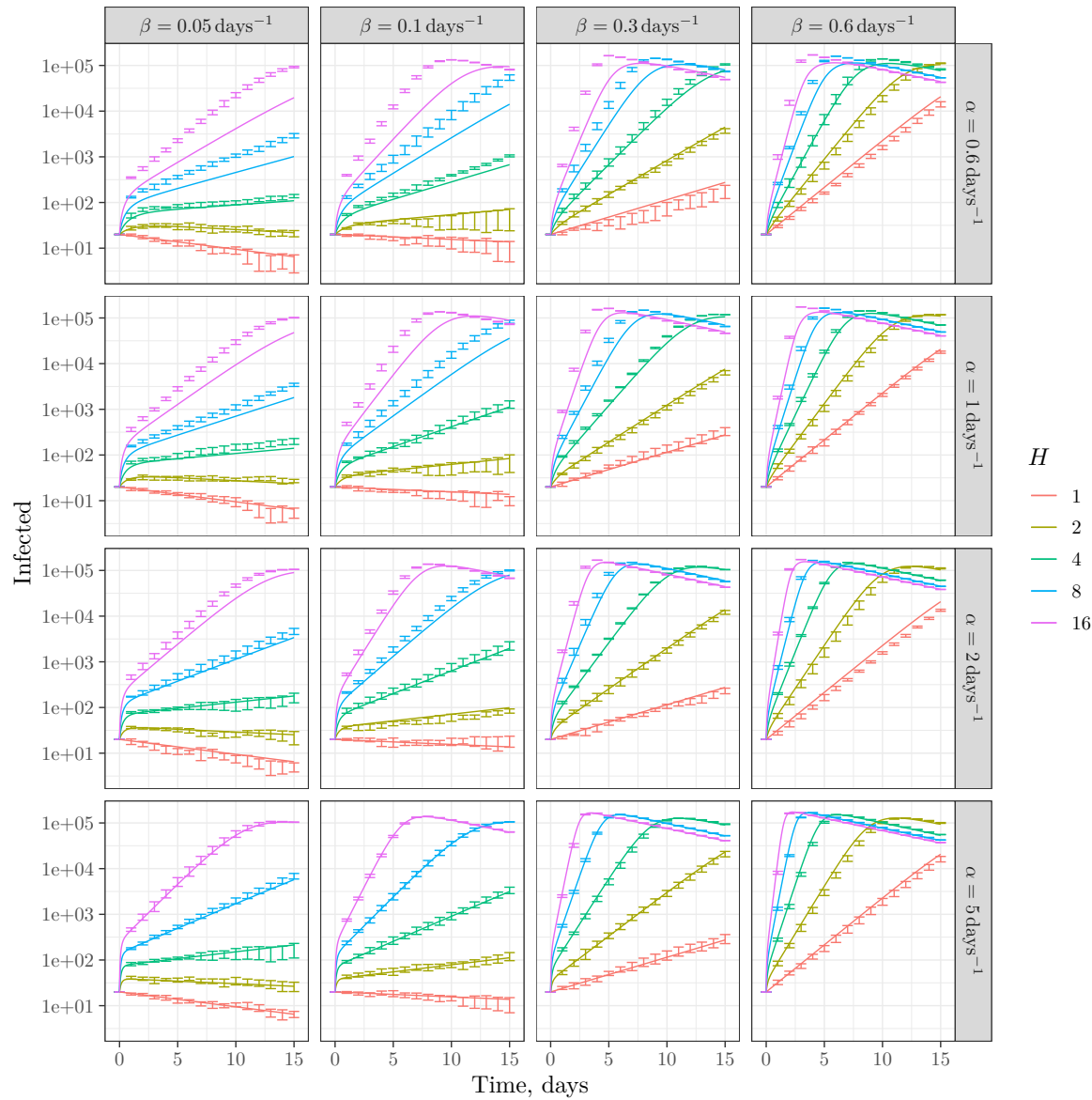
Figure 5. Simulations and mean-field predictions. The lines correspond to numerical solution of equations (1) and (2). The error bars correspond to the confidence intervals for repeated simulations computed as 1.58\text{IQR}/\sqrt{n} [20]. Each subfigure corresponds to a combination of \alpha and \beta as shown on the panels with a curve for each value of H .
