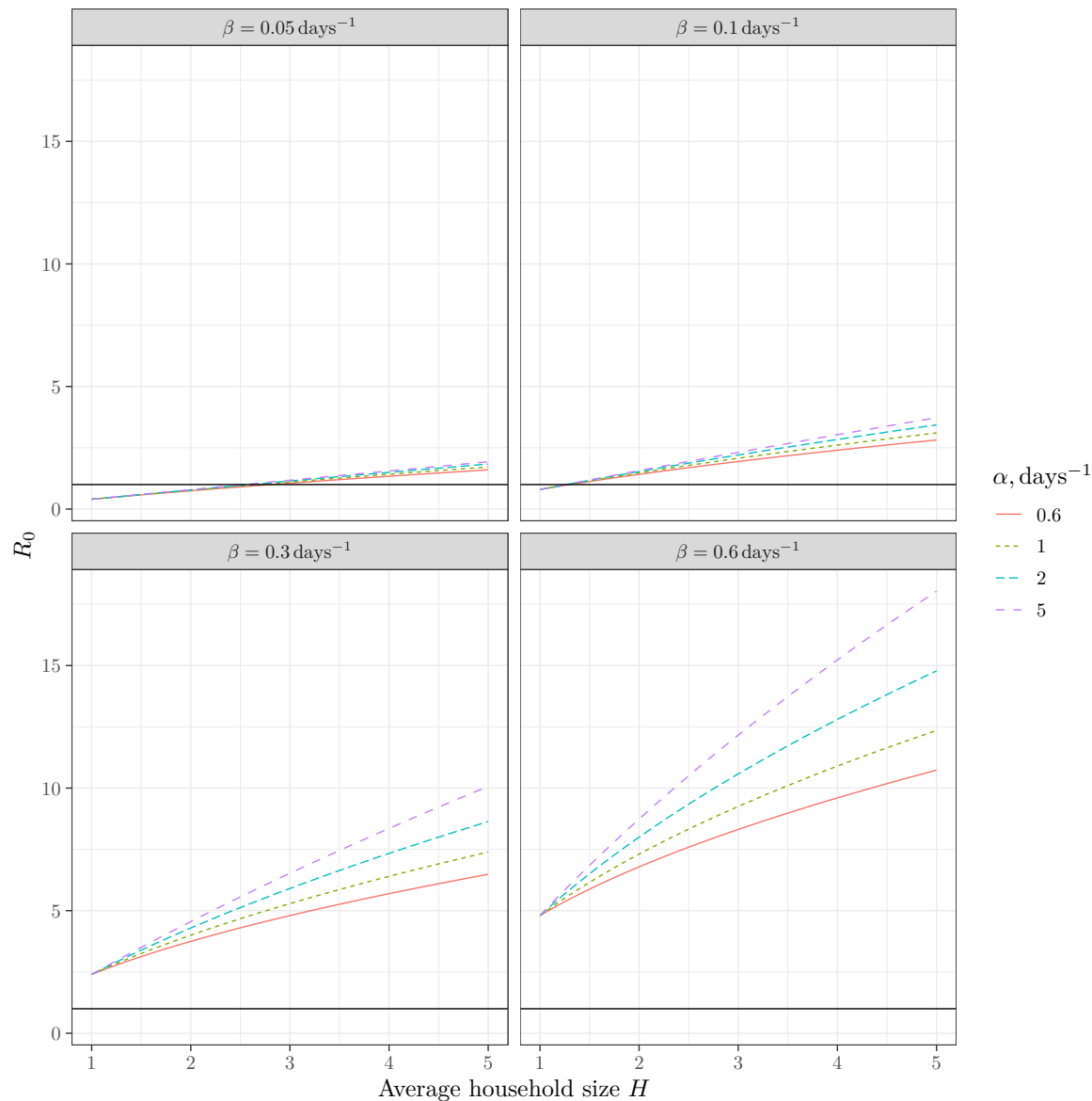
Figure 4. R_0 for the model with \gamma = 0.125 \text{ day}^{-1} . The horizontal line corresponds to R_0 = 1 . Each subfigure corresponds to a fixed \beta with a curve for each value of \alpha .
