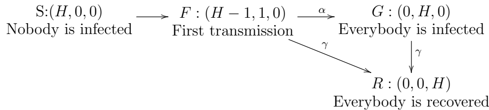
Figure 3. Simplified state diagram for a household. The household state is (s, i, r) : susceptible, infected, recovered.
