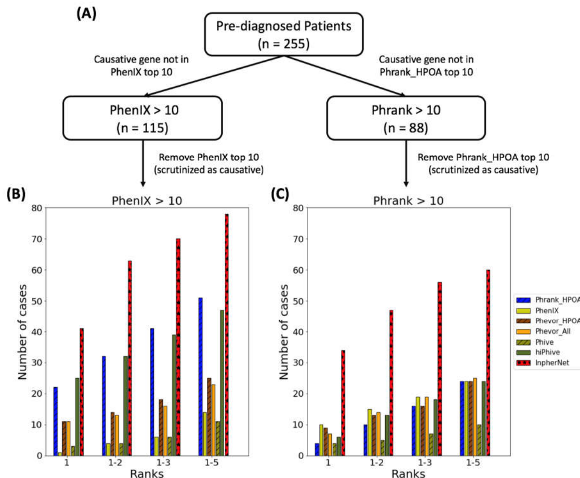
Figure 5. InpherNet outperforms existing gene prioritization methods. To mimic the clinical transition to the research inference realm (Figure 1), we took 255 patients with diverse pre-diagnosed conditions and first used two human data-only based methods to attempt quick clinical diagnosis. For 137 out of 255 patients, the causative gene was not among the top 10 output genes by at least one of the two tools. (A, left) In 115 (83.9%) of 137 cases the causative genes was not among the top 10 PhenIX-prioritized candidate genes. (A, right) In fewer cases (88 of 137, 64.2%), the causative gene was not in the Phrank_HPOA top-ranked 10 genes. Each case is then reviewed by multiple inference tools after removing the highest ranked 10 genes that were already determined to be not causai. (B) 7 different gene prioritization tools configurations were run on the remaining candidate genes (3 clinical and 4 inference tools). Since the top 10 PhenIX genes have been removed, PhenIX can still rank the causative gene high among the remaining candidate genes. However, the graph shows that most of the cases are truly difficult for the
