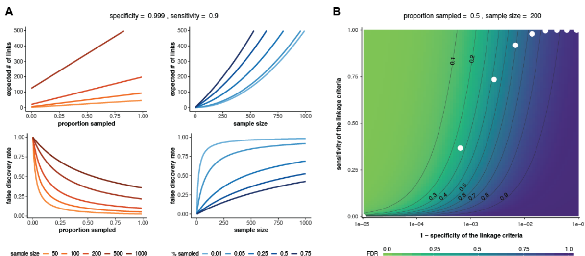
Figure 3. Sample size and false discovery rate given multiple linkage and multiple transmissions. (A) Effect of sample size (red lines) or proportion sampled (blue lines) on the expected number of linked pairs (upper plots) or the false discovery rate of linked pairs (lower plots). The specificity and sensitivity are held constant. (B) Effect of varying the sensitivity and specificity of the linkage criteria on the false discovery rate (FDR). White dots: theoretical sensitivity and specificity values at different genetic distance thresholds for a hypothetical pathogen with mutation rate = 1 mutation/genome/transmission and R=2 (see 'Determining sensitivity and specificity' below for details). In both panels, R_{pop} = 1 .
