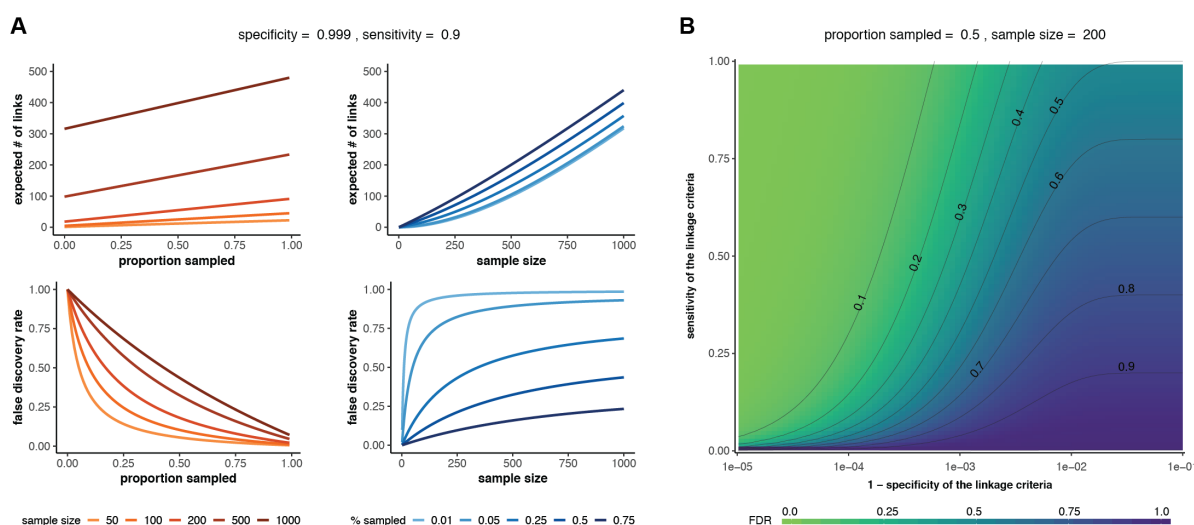
117 Figure 2. Sample size and false discovery rate given single linkage and single transmission. (A) Effect of sample size 118 (red lines) or proportion sampled (blue lines) on the expected number of linked pairs (upper plots) or the false discovery rate of 119 linked pairs (lower plots). The specificity and sensitivity are held constant. (B) Effect of varying the sensitivity and specificity of 120 the linkage criteria on the false discovery rate (FDR).
