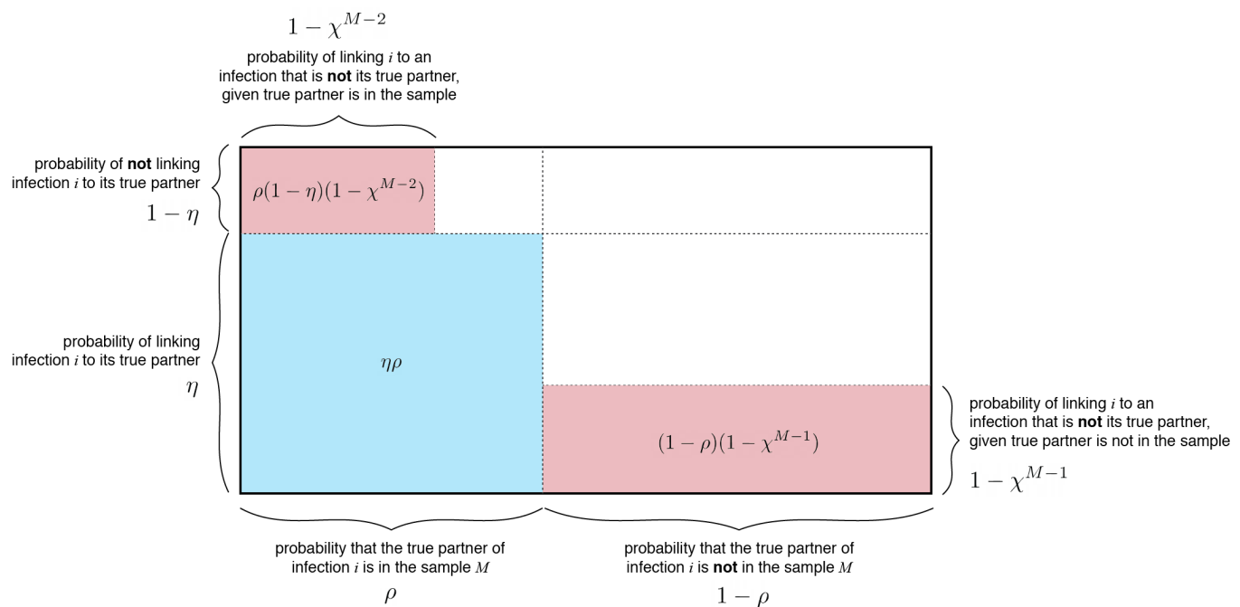
Figure 1. Visual derivation of the probability of correctly identifying a true transmission pair. Blue shaded regions represent correct identification of the true transmission partner of a random infection i . Red shaded regions represent linkage of i to an infection that is not its true transmission partner. White shaded regions represent the probability of no linkage occurring.
