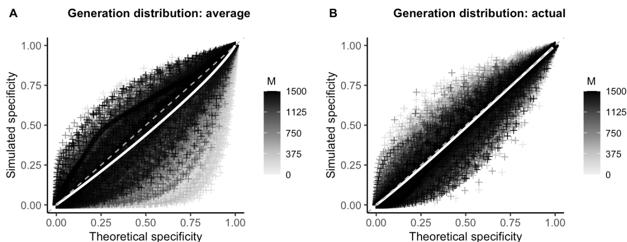
Figure 7: Effect of the generation distribution on specificity of the linkage criteria. Theoretical versus simulated specificity for each genetic distance threshold in 10,000 simulations of varying mutation rate and reproductive number (proportion sampled = 0.75). White line: smoothed conditional mean; grey dashed line: y=x line. Increasing values of the sample size ( M ) are plotted in darker color. (A) Theoretical sensitivity and specificity calculated using average distribution of generations between infections from simulations (see Text S2 ). (B) Theoretical sensitivity and specificity calculated using the actual distribution of generations between infections from that simulated outbreak.
