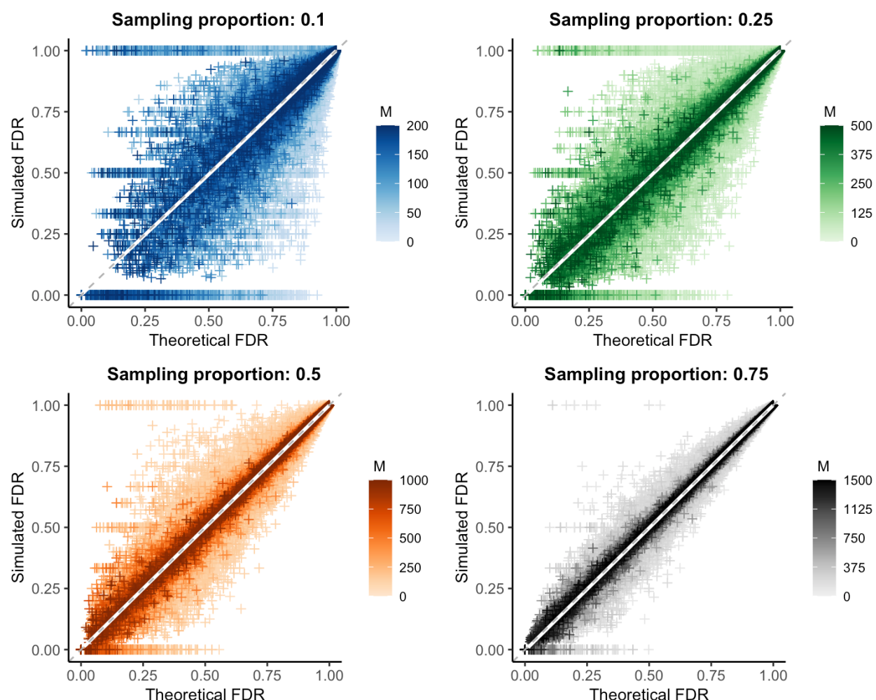
Figure 5: Predicted versus observed false discovery rate in outbreak simulations. Theoretical versus simulated false discovery rate (FDR) for each genetic distance threshold in 10,000 simulations of varying mutation rate and reproductive number. White line: smoothed conditional mean; grey dashed line: y=x line. Increasing values of the sample size ( M ) are plotted in darker color; because the maximum outbreak size is fixed at 2000, the maximum sample size differs for each sampling proportion. Increasing both the sample size and proportion reduces bias and error, see Table 2 .
