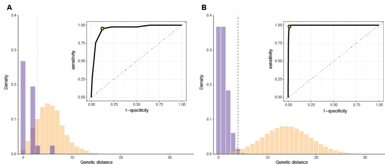
191 Figure 4. Determining the sensitivity and specificity of a genetic distance threshold. (A) Empirical distribution of genetic 192 distances for linked (purple) and unlinked (yellow) infections for 50 infections selected from early in a simulated outbreak ( \mu = 1 193 mutation/genome/generation, R=2 ). Inset: receiver operating characteristic (ROC) for all possible genetic distance thresholds. 194 Optimal threshold shown as green dot (ROC) and dashed vertical line (distribution). (B) Estimated distribution of genetic 195 distances for linked and unlinked infections generated by the mutation rate method. Parameters and plots are as in (A).
