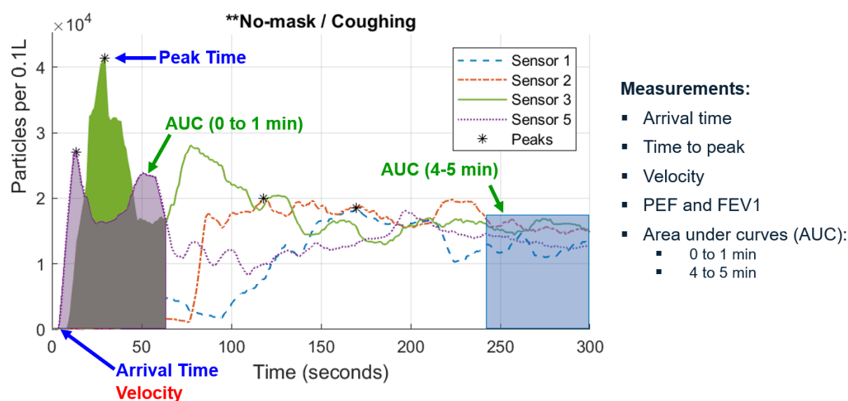
Figure 1: Examples of the measurements performed on the time-series data from all experiment runs for each of the four sensors and particle sizes of 0.3 \mu m, 0.5 \mu m, 1 \mu m, 2.5 \mu m, 5 \mu m, 10 \mu m
