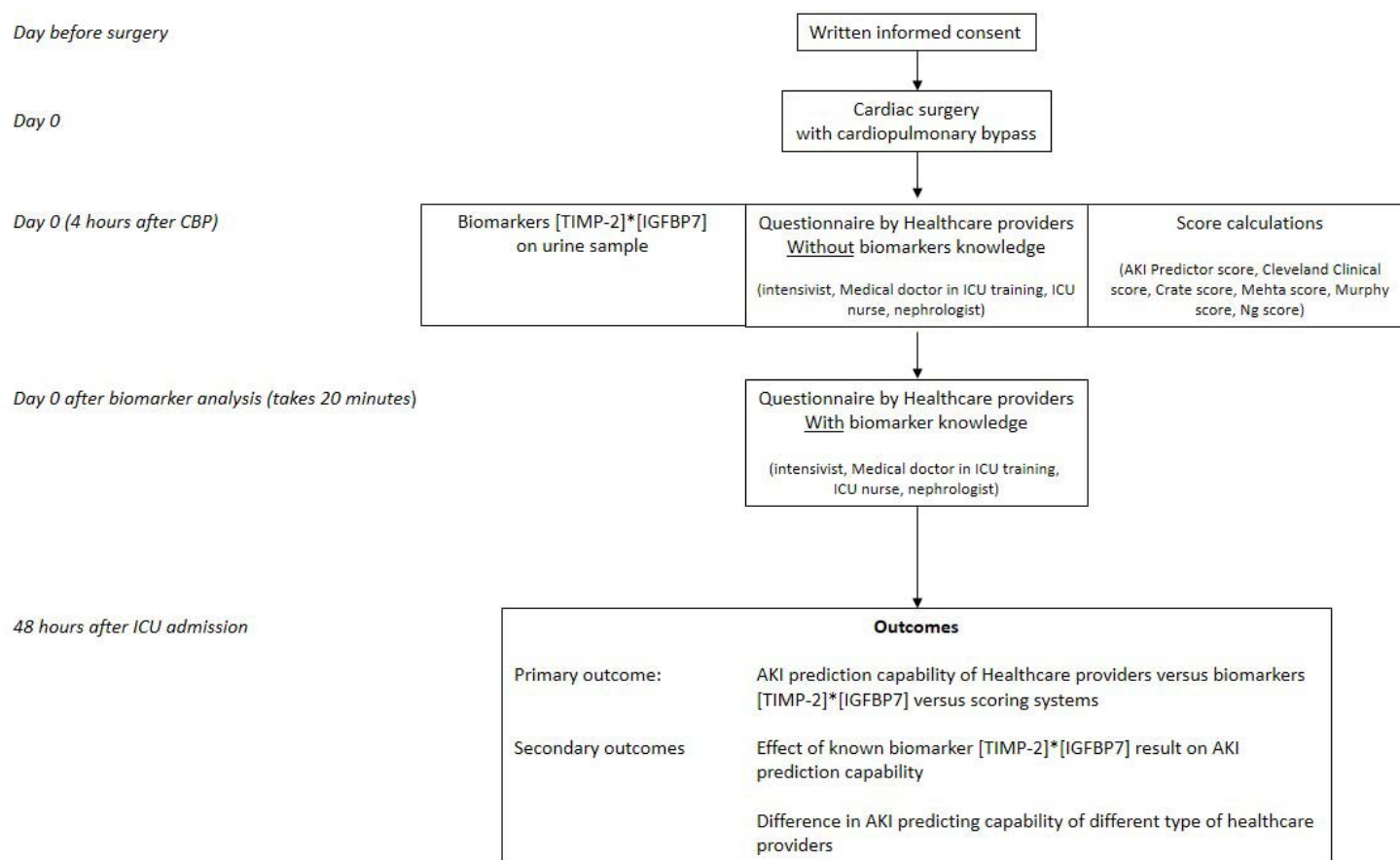
Figure 1: Trial workflow
