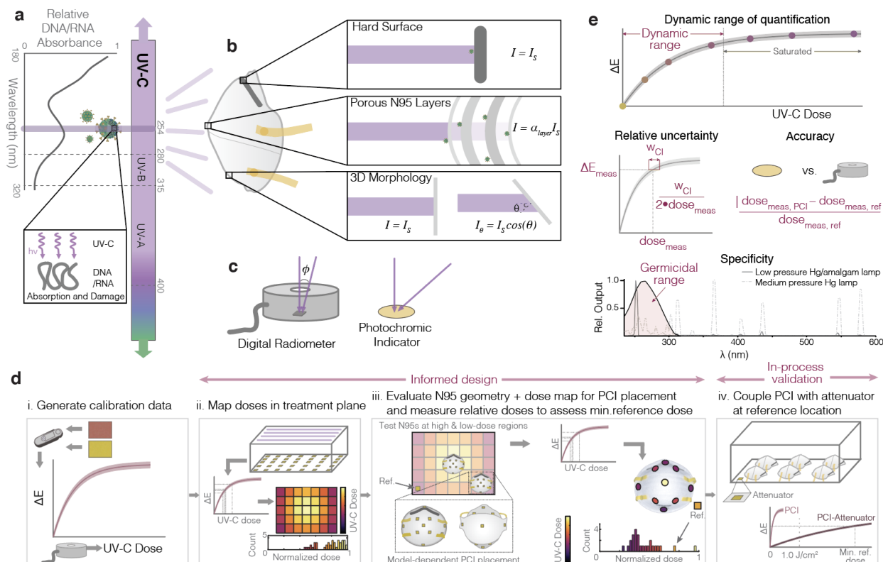
Figure 1. Mechanism and challenges of UV-C for N95 decontamination. (a) UV-C at 254 nm primarily inactivates pathogens by damaging genomic material (absorption peak near 260 nm). Nucleic acid absorbance spectrum modified from Voet et al. 25 . (b) The multilayer porous N95 materials and 3D morphology reduce the irradiance (and thus dose) available for pathogen inactivation compared to the irradiance that reaches nonporous surfaces ( I_s ), like the metal nosepiece ( \alpha_{layer} represents the layer-dependent attenuation factor). (c) UV-C detectors often have angle-dependent responses that differ from the ideal cosine response expected from a surface such as flat photochromic indicators. (d) The introduced workflow allows end-users to both design and validate their UV-C systems, reducing source- and sensor-specific inaccuracies. Critically, assessment of treatment area dose nonuniformity informs N95 placement during on-N95 measurements; on-N95 measurements in turn determine minimum reference PCI doses that yield \geq 1.0 \text{ J/cm}^2 to all N95 surfaces. On-N95 measurements are designed to specifically measure steep-angled or potentially-shadowed N95 regions (Supplementary Note 1). (e) Robust UV-C measurements must meet key specifications, including dynamic range of quantification (before the indicator saturates), relative measurement uncertainty (determined from error propagation from the confidence intervals on the calibration curve fit), accuracy of the measurement compared to a calibrated standard sensor, and specificity of the PCI response to the germicidal wavelength range (in order to accurately report germicidal activity). Specificity curves adapted from Kowalski 7 , Schmid et al. 26 , and Blickenstorfer and Aufmuth 27 . SARS-CoV-2 diagrams adapted from an image by Maya Peters Kostman for the Innovative Genomics Institute.
