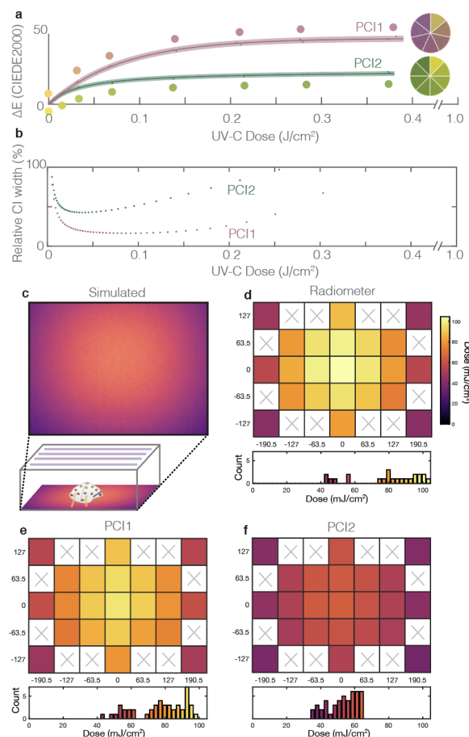
Figure 2. Robust color measurement facilitates UV-C dose quantification from two models of PCIs. (a) CIEDE2000 color difference between exposed and unexposed Intellego UVC Dosimeter Dot (PCI1, pink) and UV Process Supply UVC Intensity Label (PCI2, green) as a function of UV-C dose. Dose-responses for PCI1 were fit with a calibration function corresponding to first-order reaction kinetics (Eq. 2: R^2 = 0.998 ; a = 47.1 (46.1, 48.1); b = 80.4 (74.6, 86.3)). Dose responses for PCI2 were fit with a calibration curve corresponding to second-order reaction kinetics (Eq. 3: R^2 = 0.992 ; a = 47.7 (45.9, 49.5); b = 0.00060 (0.00049, 0.00072)). PCI color is depicted by the RM200QC-measured color values (circles) and digital SLR camera (DSLR) image swatches in the comparison wheels. Dots denote individual PCI measurements, line denotes best fit, shaded region denotes 95% confidence interval on prediction of color change from observation of UV-C dose. (b) Relative quantification uncertainties using the PCI calibration workflow. Plots depict quantified 95% confidence intervals on measurements of UV-C dose from CIEDE2000 color difference between exposed and unexposed PCIs, normalized to and as a function of UV-C dose. (c-f) heatmaps and histograms of delivered UV-C dose to locations across the treatment plane, quantified with Zemax OpticStudio simulations (c), digital radiometer (with correction factor, mean of N=3 measurements at each location) (d), PCI1 (mean of N=2 measurements at each location) (e) and PCI2 (mean of N=2 measurements at each location) (f). The PCI2 model appears to underestimate both dose and nonuniformity. Heatmaps are plotted on the same color scale (up to the radiometer maximum measured dose). White regions with 'x' in (d-f) were not measured.
