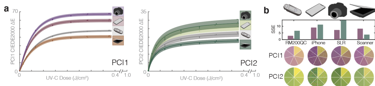
Figure 4. The potential applications for UV-C quantification from PCIs could be broadened using widely-available color measurement tools. (a) Comparison of calibration curve fits of CIEDE2000 \Delta E from an unexposed sensor vs. UV-C dose, for PCI1 and PCI2 colors quantified using the digital SLR and iPhone X in a light box, RM200QC spectrophotometer, and flatbed scanner. Dots denote individual PCI measurements, line denotes best fit, shaded region denotes 95% confidence interval on prediction of color change from observation of UV-C dose. (b) Squared sum of the residuals (SSE) for each curve fit in (a), along with color comparison wheels showing indicator color at various doses as captured by the different imaging devices. Quantification of the dose-dependent relative uncertainty for each of the 8 curve fits is presented in Supplementary Figure S11.
