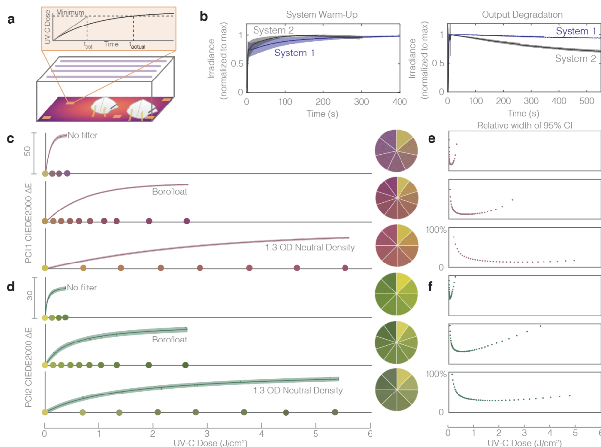
Figure 5. Quantitative in-process UV-C dose validation of N95 decontamination cycles using PCIs could be feasible using optical attenuation to extend the dynamic range beyond 1.0 J/cm 2 . (a) Treatment times calculated from single ‘snap-shot’ dose measurements inaccurately assume constant irradiance over time by disregarding bulb warm-up and thermal output degradation during exposure. (b) Two near-identical UV-C exposure systems have significantly different output profiles over time, both during warm-up (left), and during long exposures (right). Plots depict mean (line) and standard deviation (shaded region) of the measurements reported in Supplementary Figure S12. (c-d) 1.1 mm thick Borofloat™ glass and 1.3 OD neutral density filters extend the dynamic range of PCI1 (c) and PCI2 (d) sensors. PCI1 no filter R 2 = 0.998, a = 47.1, b = 80.4. PCI1 with Borofloat™ filter R 2 = 0.999, a = 47.3, b = 699. PCI1 with 1.3 OD neutral density filter R 2 = 0.998, a = 44.2, b = 2728. PCI2 no filter R 2 = 0.992, a = 47.7, b = 0.00060. PCI2 with Borofloat™ filter R 2 = 0.990, a = 61.8, b = 3.63x10 -5 . PCI2 with 1.3 OD neutral density filter R 2 = 0.992, a = 62.7, b = 1.10x10 -5 . Color comparison wheels show PCI colors corresponding to doses marked along the x-axis, except in “No Filter” cases due to space constraints on the x-axis. Dots denote individual PCI measurements, line denotes best fit, shaded region denotes 95% confidence interval on prediction of color change from observation of UV-C dose. The relative width of quantified 95% confidence intervals on UV-C dose measurements from CIEDE2000 color difference between exposed and unexposed samples of PCI1 (e) and PCI2 (f), as a function of UV-C dose, plotted to the right of corresponding dose-response curve.
