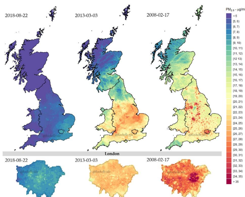
Figure 4: Stage-4 day-specific PM 2.5 estimations across Great Britain (Top) and London (Bottom).
