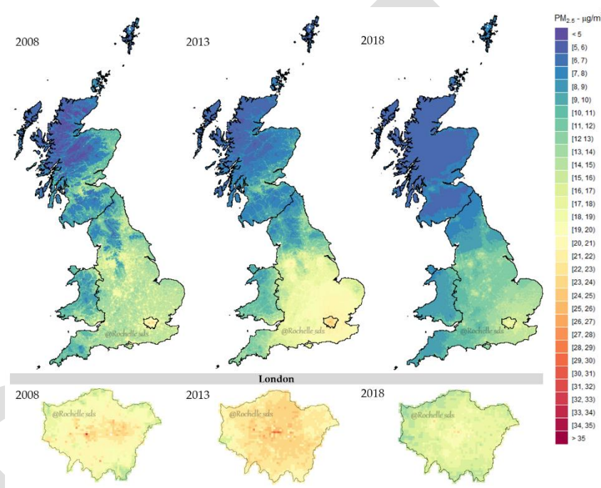
Figure 3: Stage-4 predicted \text{PM}_{2.5} concentrations across Great Britain (Top) and London (Bottom) for 2008, 2013, and 2018 aggregated by annual means. All plots were built under the same colour scale.
