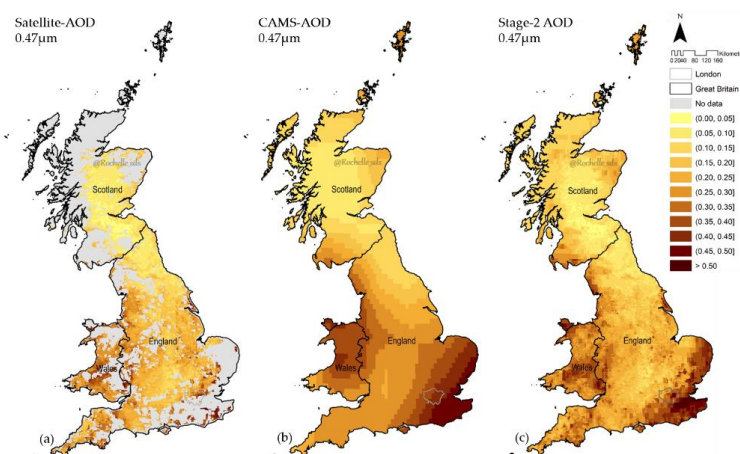
Figure 2: Satellite-AOD 0.47\mu\text{m} values are represented in Figure 2a (mean of all Terra- and Aqua-MODIS passing times). The missing values in grey were imputed through a combination of multiple modelled-AOD wavelengths and sub-day times, represented in Figure 2b by modelled-AOD 0.47\mu\text{m} at 12:00. Stage-2 output is shown in Figure 2c, illustrating the full coverage of AOD 0.47\mu\text{m} based on the combination of measurements and estimations across Great Britain. The maps correspond to values measured or reconstructed on 6th July 2018.
