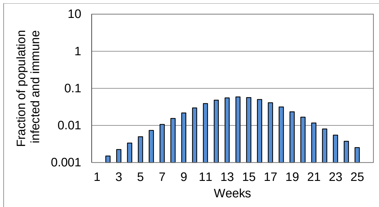
Fig. 2 – Simulation of weekly new case infections that confer “permanent” immunity and eradication of the virus: R_0 = 1.5 , A = 1
