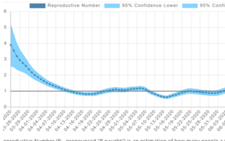
Fig. 6 – Derived CoV-2 infection rate history for St. Louis, MO [5].
