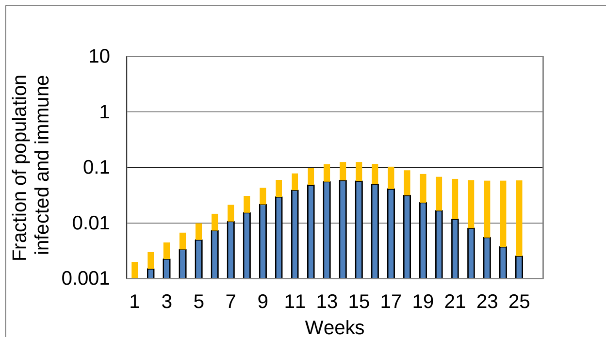
Fig. 3 - Permanent immunity (blue) compared to limited duration immunity (orange) for R_0 = 1.5 , A = 1 .
