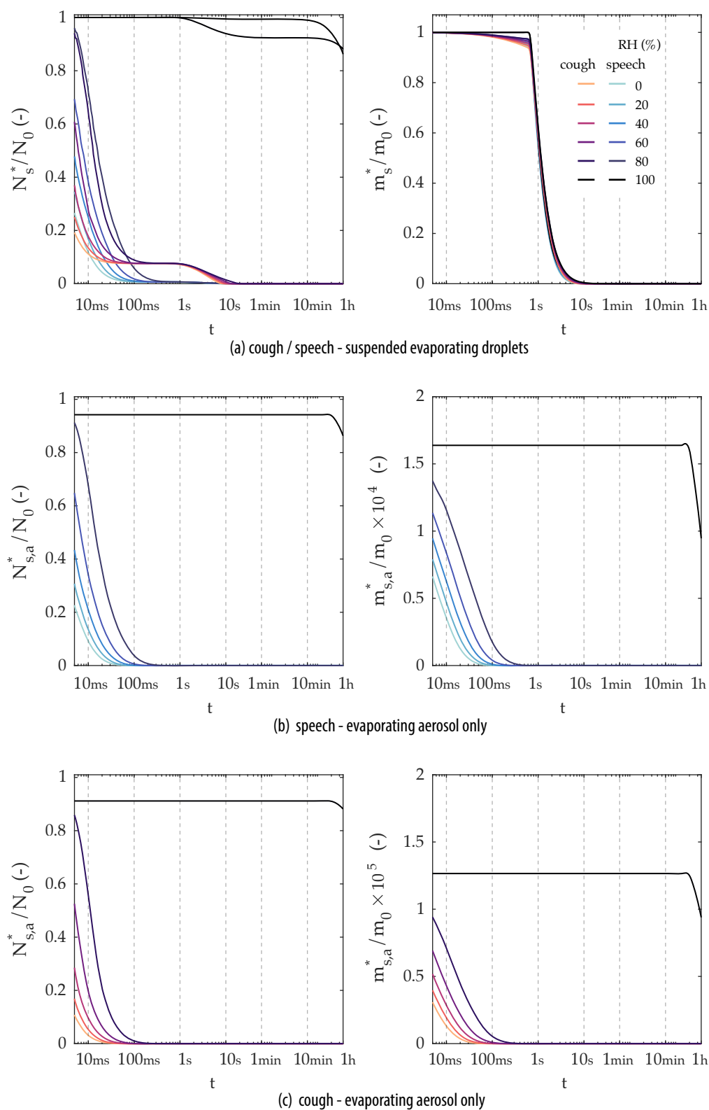
Figure 7. Time evolution of ensemble quantities (total mass and number) normalised by the respective value at t = 0 for sprays exhaled by speech and cough – T=20^\circ\text{C} , \text{RH}=0\text{--}100\% . The quantities only consider evaporating droplets, that is, droplets that have not yet achieved equilibrium with ambient air. In the lower row, ensemble quantities shown are calculated considering only droplets below 5\text{ }\mu\text{m} .
