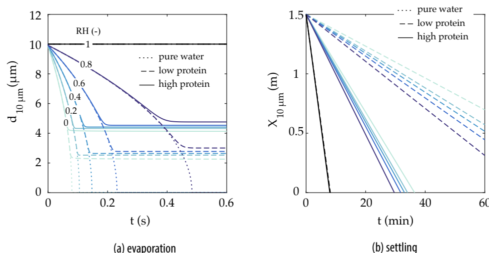
Figure 8. Impact of the droplet composition modelling approach (pure water; sputum 9 mg/ml NaCl, 3 mg/ml protein; sputum 9 mg/ml NaCl, 76 mg/ml protein) on the (a) evaporation and (b) settling of 10 µm droplets under different relative humidities. The relative humidity is shown in colour (RH=0–100%) – T=20°C.
