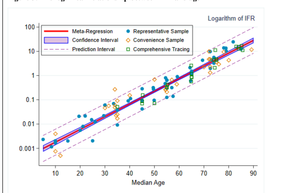
Figure 3: The log-linear relationship between IFR and age
