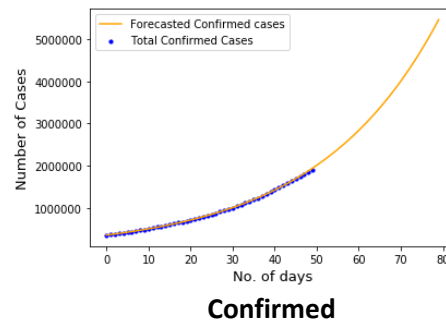
Figure 4. Forecasting plots for exponential curve fitting
