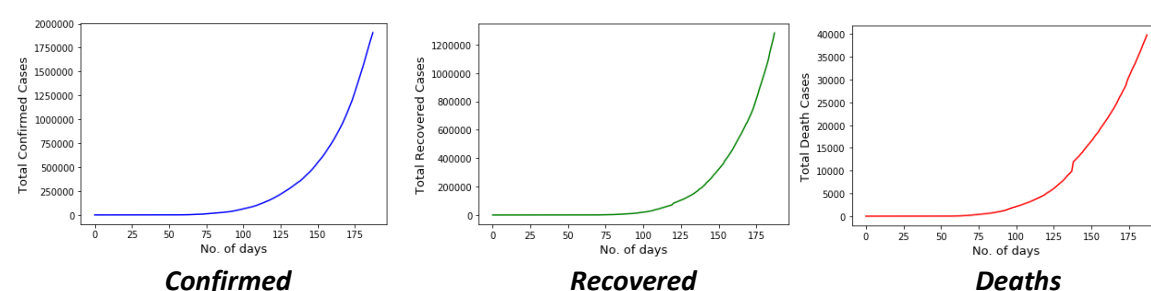
Figure 1. Plots of cumulative cases in India
