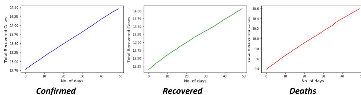
Figure 2. Plots of natural logarithm of cumulative cases in India
