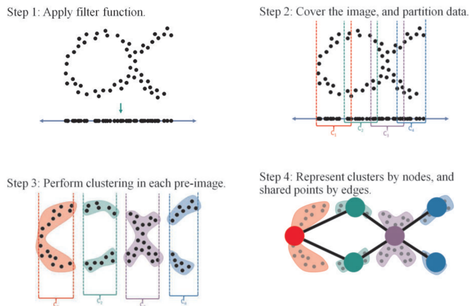
FIGURE 1. An illustration of the Mapper algorithm. Image Source: Escolar, Hiraoka, Igami, Ozcan [7].
