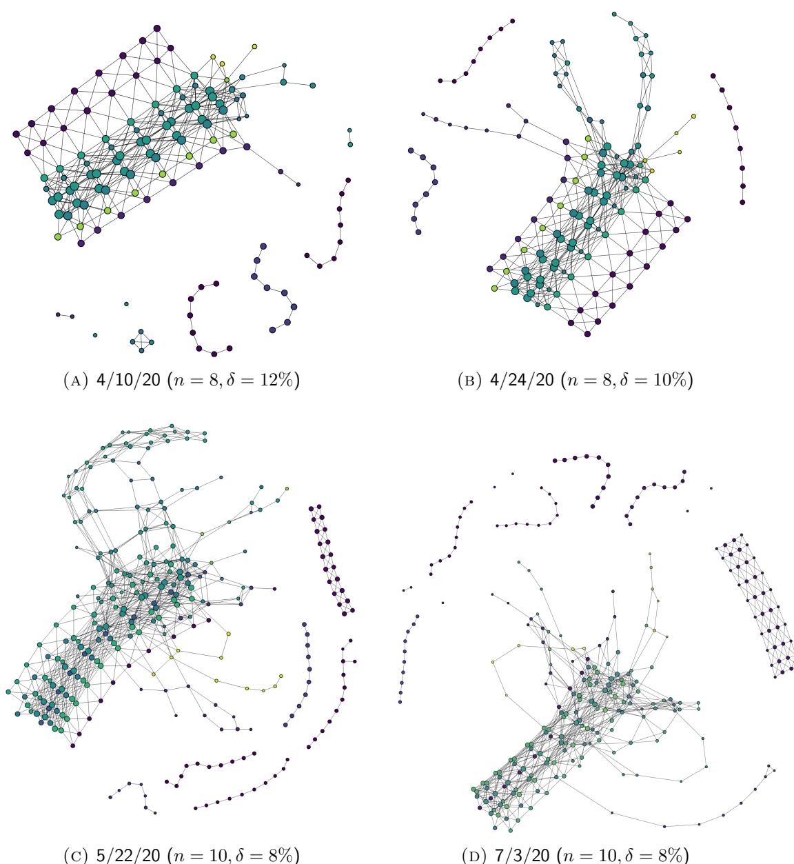
FIGURE 12. The evolution of Mapper graphs over time for filtered data (see Section 2.3.1).
