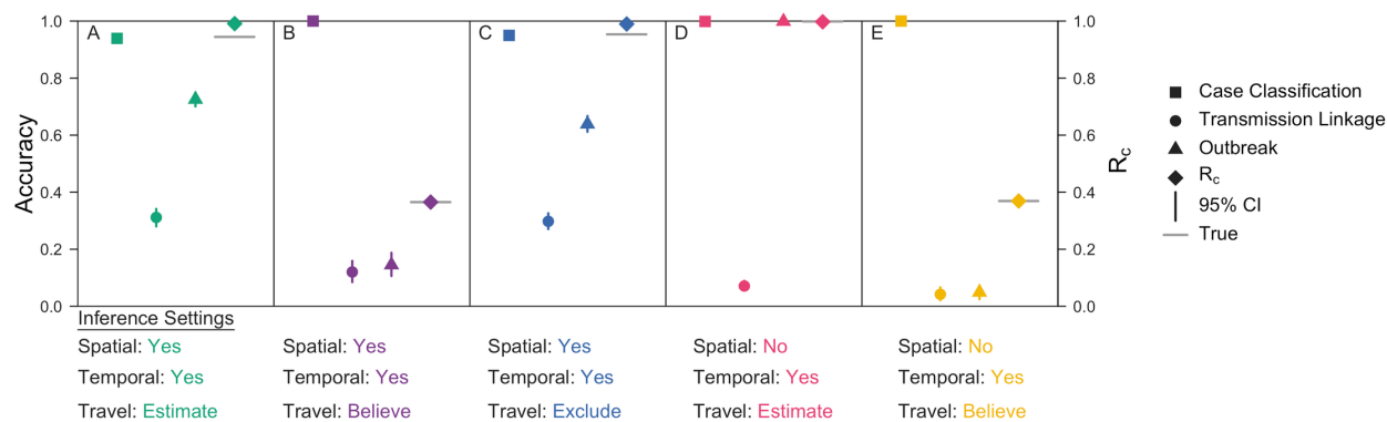
Fig 6. Inference accuracies for validation exercises. Accuracy metrics are reported for each inference setting applied to its respective simulated data set. Case Classification, represented by squares, refers to the proportion of cases that are correctly classified as imported or locally acquired. Transmission Linkage, denoted by circles, is the proportion of locally acquired cases for which the true parent is correctly identified. Outbreak, represented by triangles, is the proportion of locally acquired cases for which the inferred parent belongs to the correct outbreak. Bars denote the 95% credible intervals, and the grey line is the true R_c value of the network.
