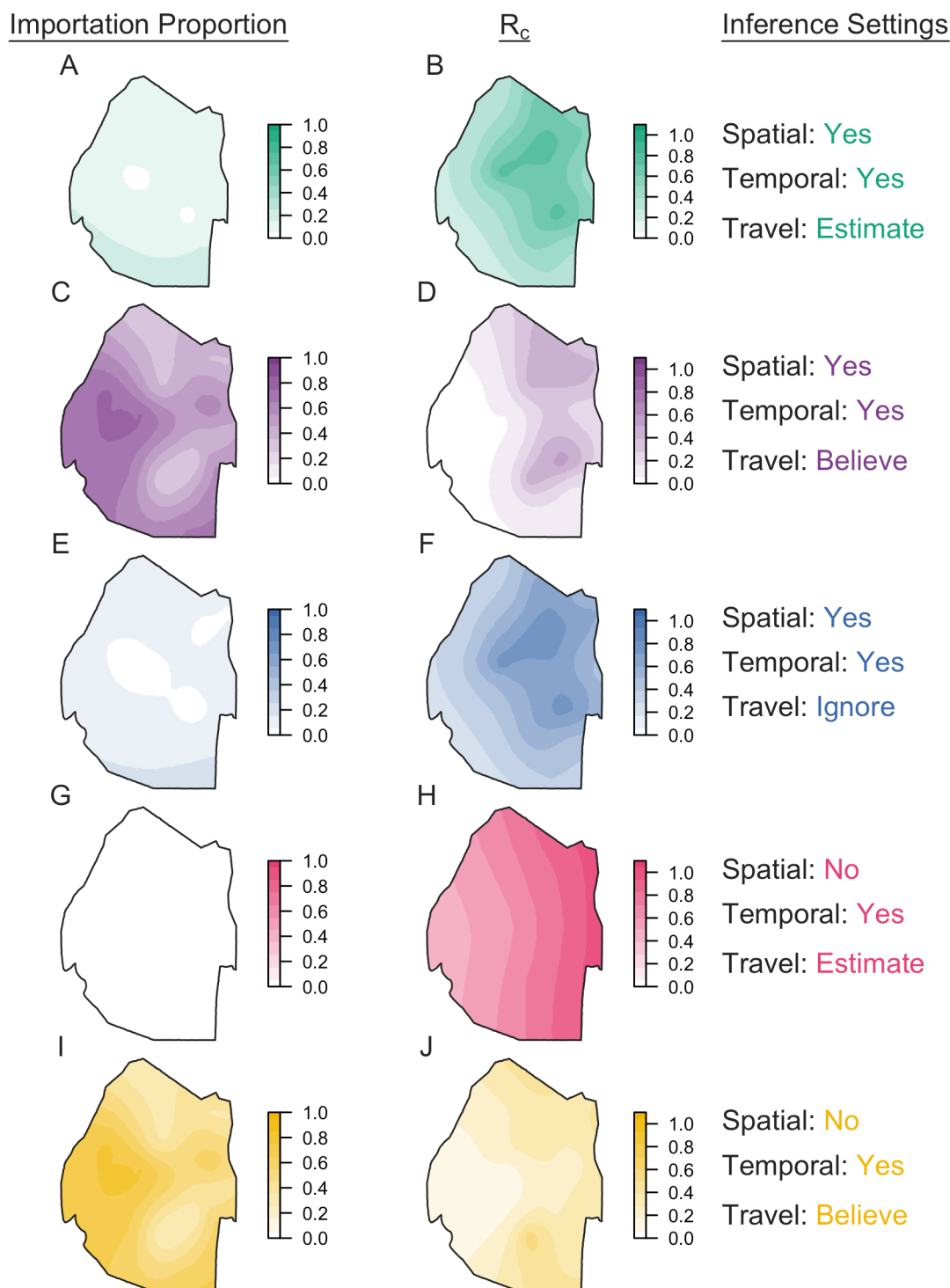
155 156 Fig 3. Spatial distribution of importation and transmission risk in Eswatini. Maps of the 157 proportion of cases that are imported and the reproduction number under control ( R_c ) were
