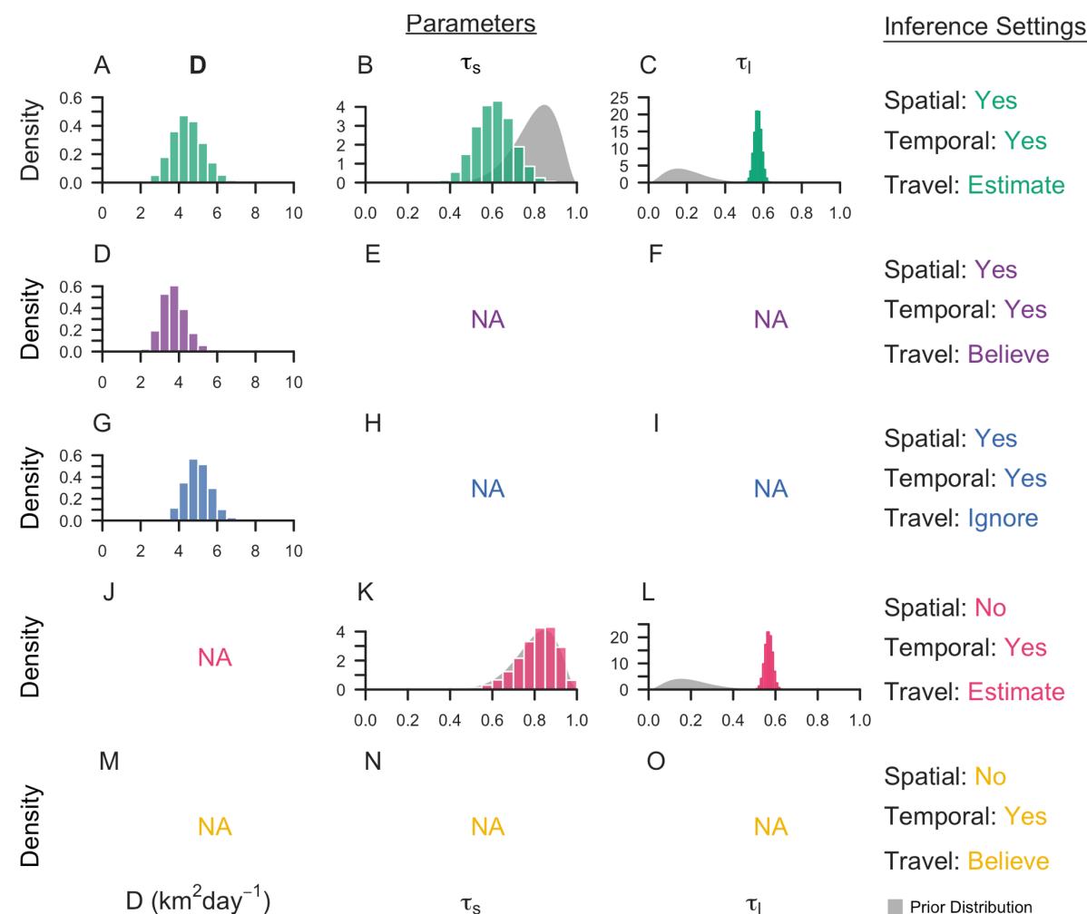
Fig 1. Marginal posterior distributions of parameters from Eswatini surveillance data.
