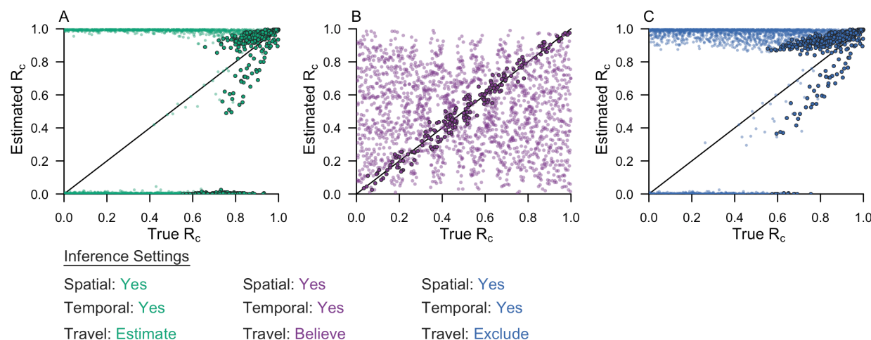
Fig 7. Comparison of R_c estimates across inference settings. The inference algorithm was applied to 2,000 simulated data sets. The estimated R_c is compared to the true R_c for each of the inference settings: (A) spatial and temporal data while estimating the accuracy of the travel history; (B) spatial and temporal data while believing the travel history; and (C) spatial and temporal data alone. Each point represents a simulated data set. The darker, accented points are simulated data sets with epidemiological features that improved performance. In (A) and (C), the darker, accented points were simulated data sets where the mean temporal interval between imported infections was greater than two times the mean serial interval. In (B), the darker, accented points were simulated data sets where the proportion of cases reporting travel was within 0.05 of the proportion of imported cases.
