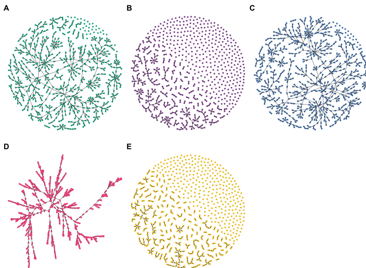
Fig 4. Maximum a posteriori transmission networks in Eswatini. The maximum a posteriori transmission networks (i.e., the transmission network in the posterior distribution with the highest likelihood) is shown for each inference setting: (A) spatial and temporal data while estimating the accuracy of the travel history; (B) spatial and temporal data while believing the travel history; (C) spatial and temporal data alone; (D) temporal data while estimating the accuracy of the travel history; and (E) temporal data while believing the travel history. In each transmission network, circles represent nodes, and arrows represent directed edges.
