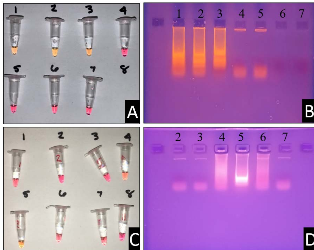
Figure 3. (A) Colorimetric reaction vessels for primer set 1.0 with the following reaction vessel containments: 1 – Primer w/DNA, 2 – Primer w/DNA, 3 – Primer w/DNA, 4 – Primer w/o DNA, 5 – Primer w/o DNA, 6 – No Primer/DNA, 7 – No Primer/DNA. (B) Ethidium bromide electrophoresis gel with samples of panel (A). The containments of each lane correspond with the reaction vessels as indicated. (C) Temperature gradient assay for LAMP primer set 1.0. Each of the reaction vessels (left) were also run with negative controls, not pictured. Reaction vessel numbers correspond with the ethidium bromide gel pictured in box (D), with the exception of vessel (1) and (8). From vessel (1) to (8), the temperature gradient follows the order (in °C): 70.8, 69.3, 67.8, 64.8, 59.3, 57.8, 56.3, and 54.8.
