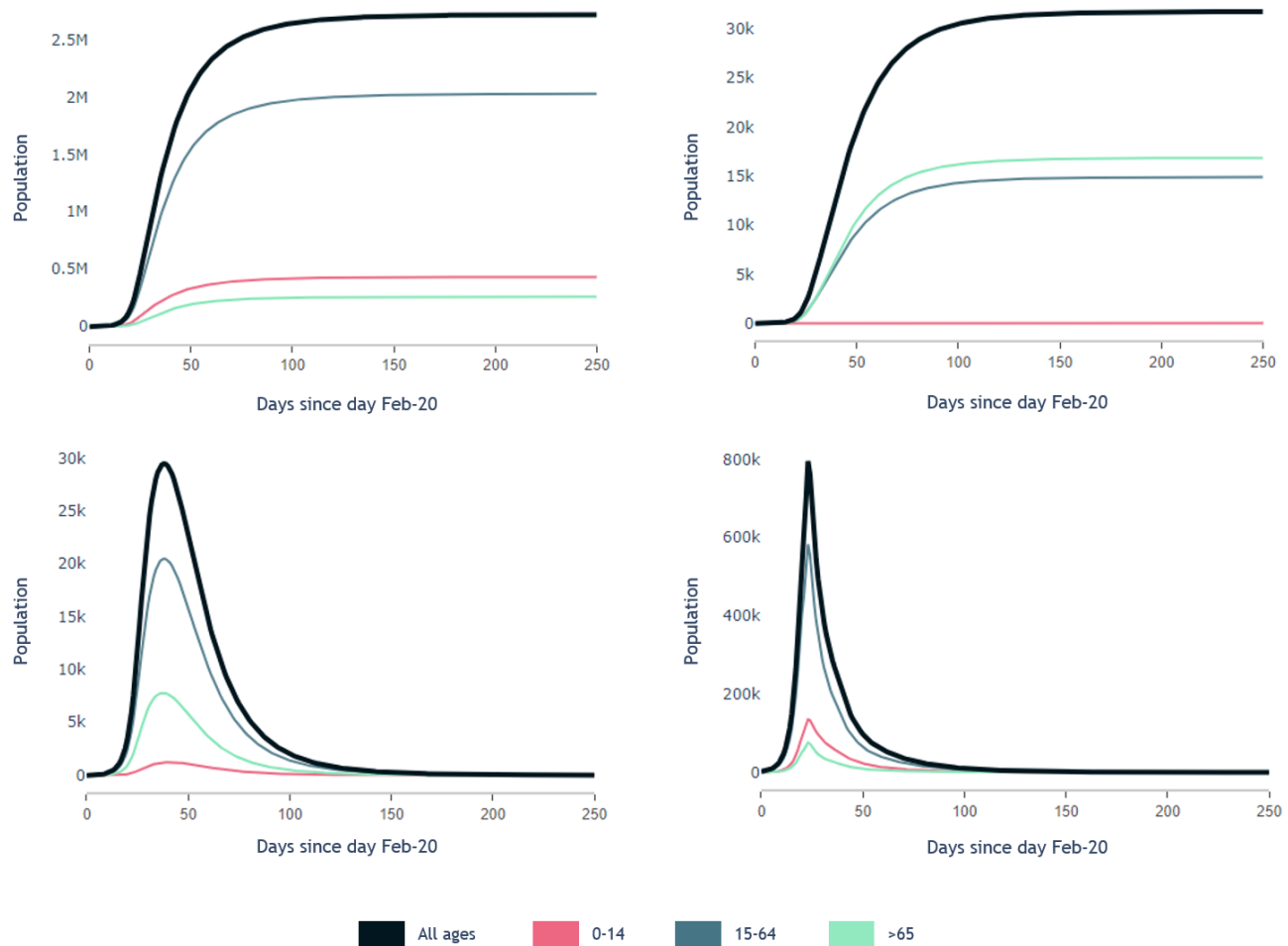
Figure 4. Scenario 2. Mobility restricted up to 30% of movements and contained during the following 250 days. From left to right, up to down, first graph shows accumulated number of people who recovered after contracting COVID-19, second graph shows accumulated number of people who deceased by COVID-19, third graph shows instantaneous number of people making use of health services and fourth graph shows instantaneous asymptomatic people.
