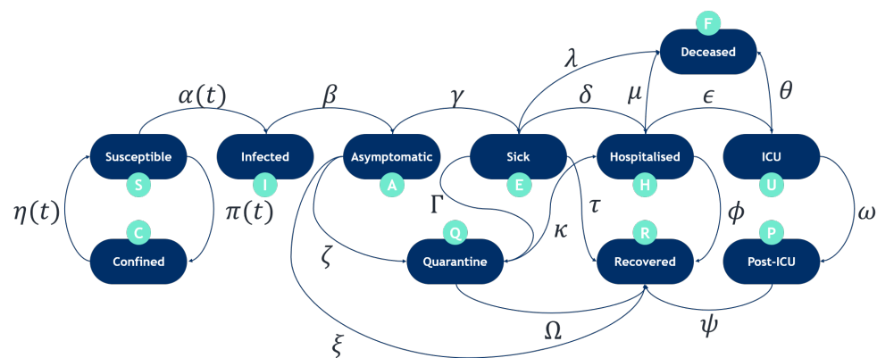
Figure 2. Epidemiological model. The epidemiological model forms the central core between the population mobility model, government interventions and possible disease evolution scenarios. It is composed of a total of eleven states.
