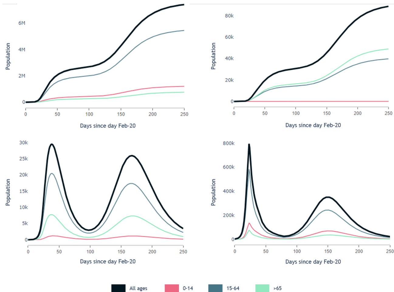
Figure 3. Scenario 1. Mobility restricted up to 30% of movements and later released up to 75%. From left to right, up to down, first graph shows accumulated number of people who recovered after contracting COVID-19, second graph shows accumulated number of people who deceased by COVID-19, third graph shows instantaneous number of people making use of health services and fourth graph shows instantaneous asymptomatic people.
