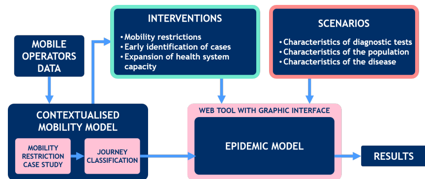
Figure 1. high-level block diagram. The epidemiological model forms the central core between the population mobility model, government interventions and possible disease evolution scenarios, leading to predictive results for the future.
