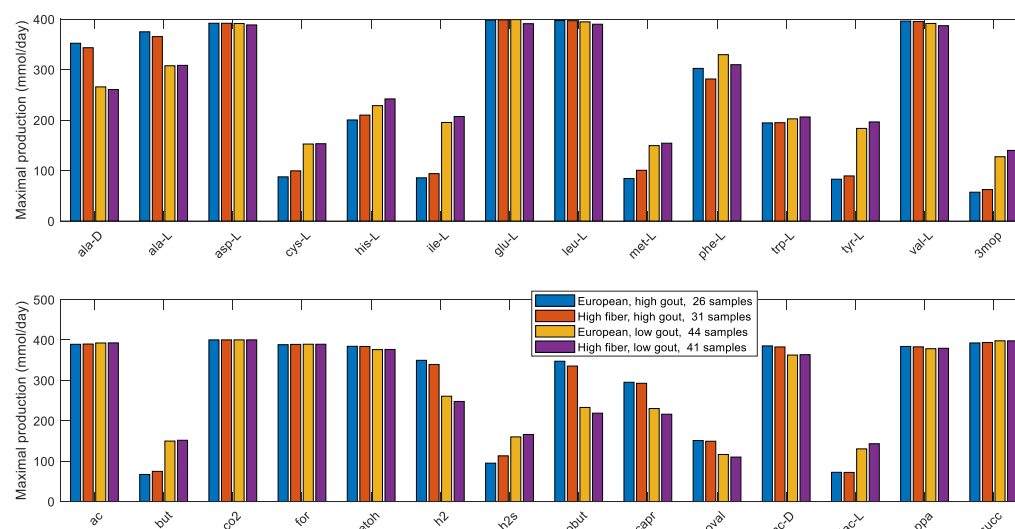
Figure S9. Maximal amino acid and fermentation byproduct synthesis capabilities in the high and low gout clusters from average EU and high fiber diets. (A) Classes of amino acids sharing common metabolic pathways. (B) Common metabolic byproducts of carbohydrate fermentation and amino acid catabolism. Metabolite abbreviations are taken from the VMH database ( www.vmh.life ).
