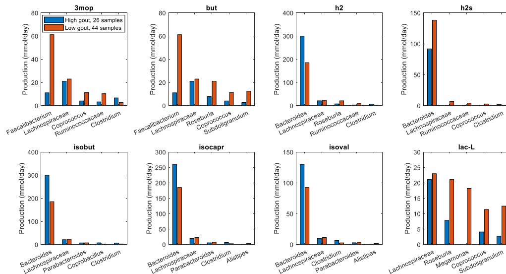
Figure 4. Individual taxa contributions to maximal synthesis of fermentation byproducts differentially produced between the high and low gout clusters from an average EU diet.
