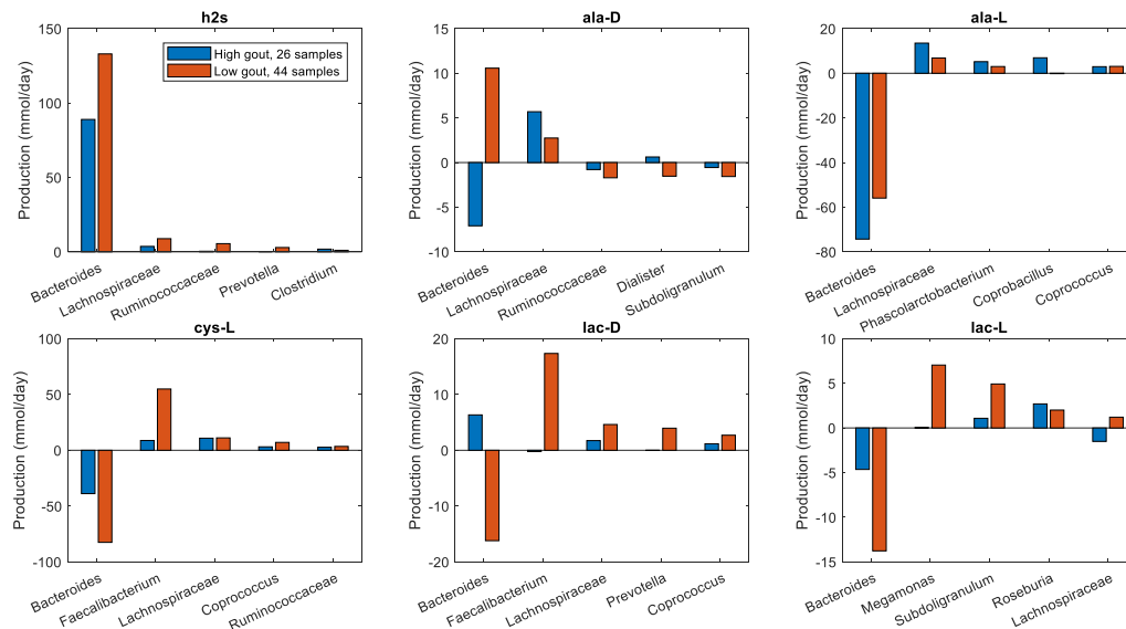
Figure 6. Individual taxa synthesis and uptake of crossfed metabolites for maximal H 2 S production from an average EU diet.
