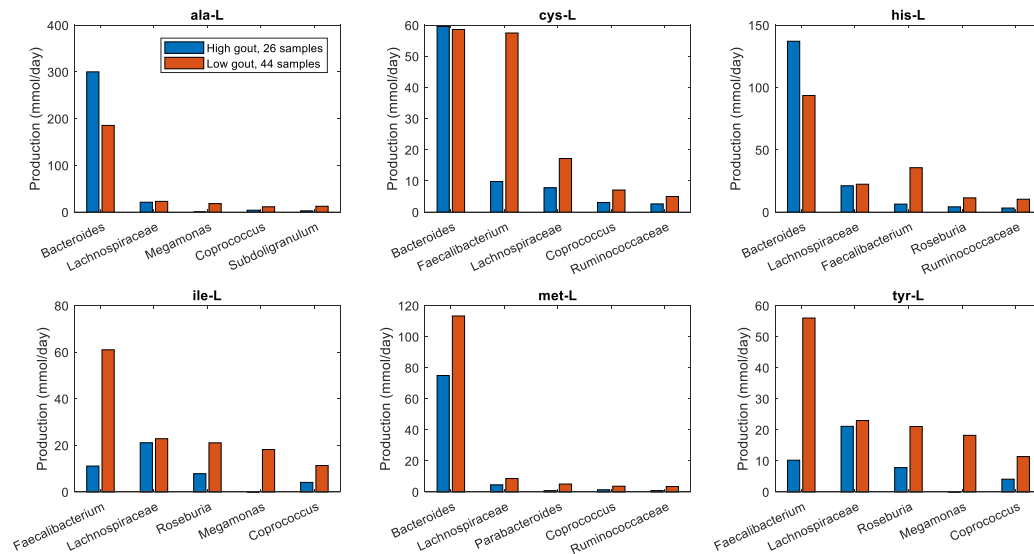
Figure 3. Individual taxa contributions to maximal synthesis of amino acids differentially produced between the high and low gout clusters from an average EU diet.
