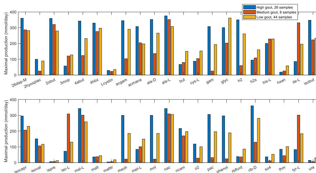
Figure S2. Differentially produced metabolites between the high and low gout clusters with an average EU diet. Significant differences in maximal metabolite production rates were determined by applying the Wilcoxon rank sum test ( FDR < 0.05 ) to each metabolite across all samples in the two clusters. In addition to being statistically different, each metabolite shown had an average production rate > 10 mmol/day in at least one cluster and average production rates that differed between the clusters by at least 10%. Metabolite abbreviations are taken from the VMH database ( www.vmh.life ). Full metabolite names, their associated metabolic pathways and numeric values for their average production rates in each cluster are given in Table S6.
