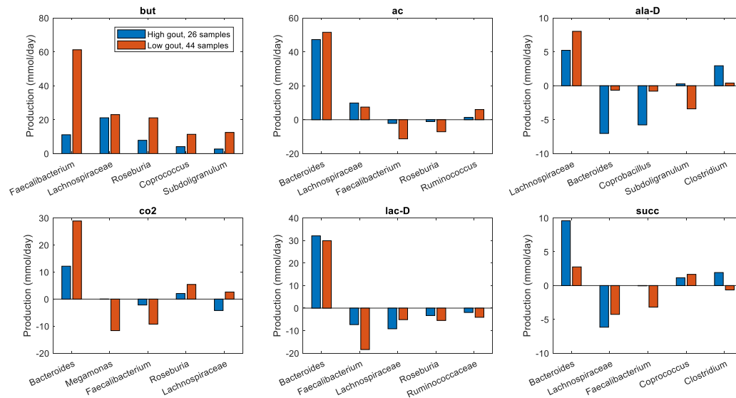
Figure 5. Individual taxa synthesis and uptake of crossfed metabolites for maximal butyrate production from an average EU diet.
