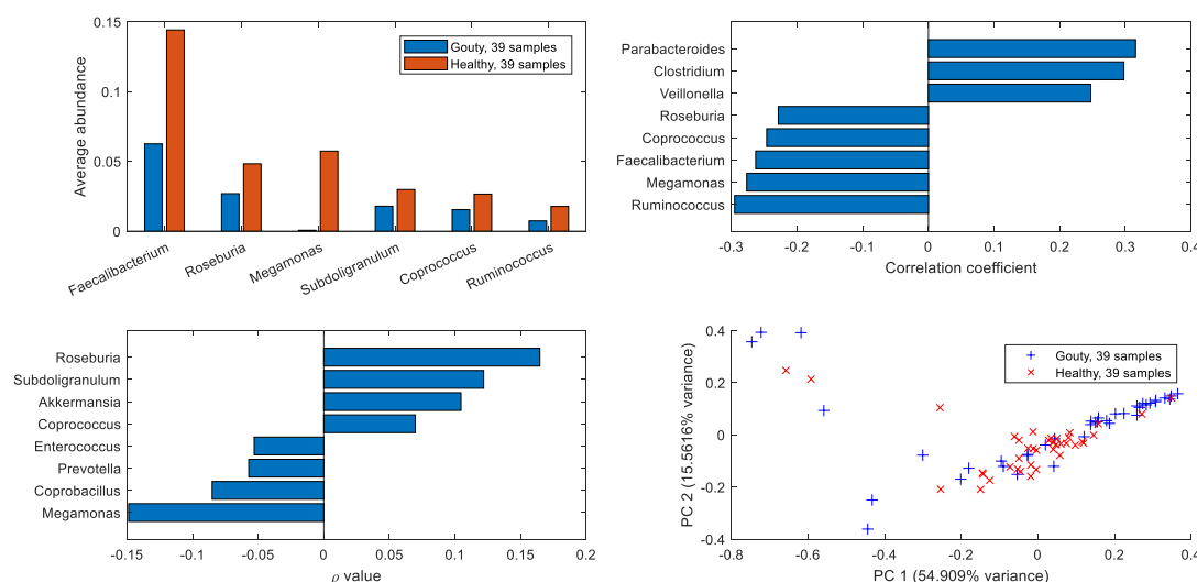
Figure S1. Analysis of normalized 16S-derived abundance data for samples in which the modeled taxa accounted for at least 90% of the unnormalized abundances. (A) Taxa which were significantly ( FDR < 0.05 ) more abundant in one sample type versus the other sample type among the 25 most abundant taxa across the 78 samples used. (B) Taxa most highly correlated with the blood uric acid concentration. (C) Taxa with the highest proportionality to Faecalibacterium . (D) Principal component plot of the 16S-derived abundance data showing gouty and healthy patient samples.
