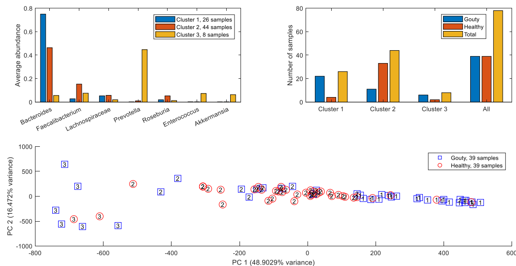
Figure 1. Clustering of model-processed 16S abundance data with an average EU diet.
