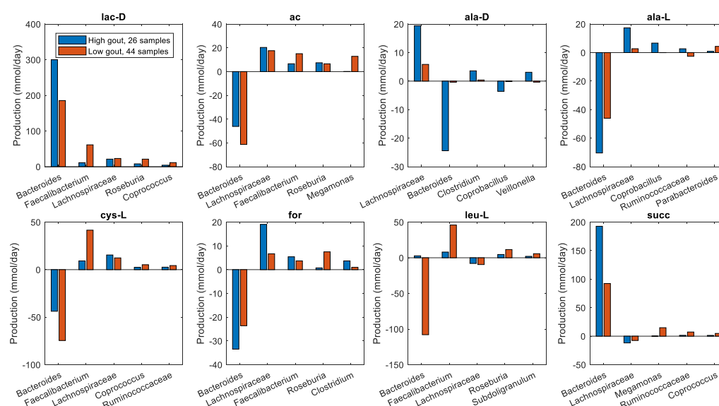
Figure S5. Individual taxa synthesis and uptake of crossed metabolites for maximal D-lactate production from an average EU diet. The metabolites shown from top left to bottom right are D-lactate, acetate, D-alanine, L-alanine, L-cysteine, formate, L-leucine and succinate. Each crossed metabolite shown had at least one taxa which satisfied minimal bounds on the metabolite secretion and uptake rates. For each metabolite, the top five taxa were ordered by the sum of the absolute values of their uptake and secretion rates across the two clusters.
