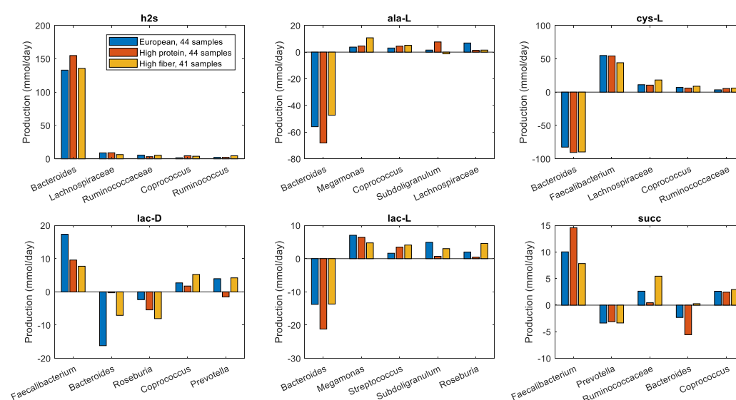
Figure S9. Maximal amino acid and fermentation byproduct synthesis capabilities in the high and low gout clusters from average EU and high fiber diets. (A) Classes of amino acids sharing common metabolic pathways. (B) Common metabolic byproducts of carbohydrate fermentation and amino acid catabolism. Metabolite abbreviations are taken from the VMH database ( www.vmh.life ).
