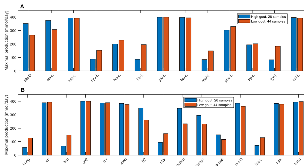
Figure 2. Maximal amino acid and fermentation byproduct synthesis capabilities in the high and low gout clusters from an average EU diet.
