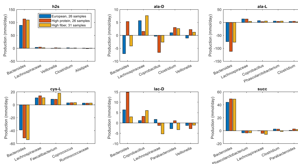
Figure 8. Individual taxa synthesis and uptake of crossfed metabolites for maximal H 2 S production in high gout clusters generated from average European, high protein and high fiber diets.
