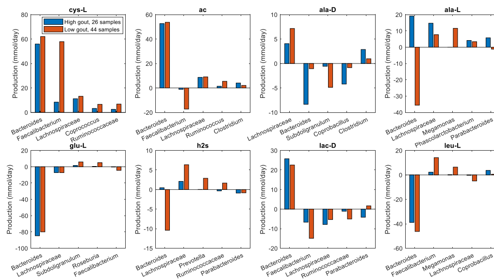
Figure S6. Individual taxa synthesis and uptake of crossfed metabolites for maximal L-cysteine production from an average EU diet. The metabolites shown from top left to bottom right are L-cysteine, acetate, D-alanine, L-alanine, L-glutamate, hydrogen sulfide and L-leucine. Each crossfed metabolite shown had at least one taxa which satisfied minimal bounds on the metabolite secretion and uptake rates. For each metabolite, the top five taxa were ordered by the sum of the absolute values of their uptake and secretion rates across the two clusters.
