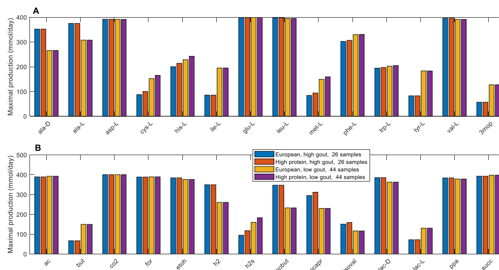
Figure S8. Maximal amino acid and fermentation byproduct synthesis capabilities in the high and low gout clusters from average EU and high protein diets. (A) Classes of amino acids sharing common metabolic pathways. (B) Common metabolic byproducts of carbohydrate fermentation and amino acid catabolism. Metabolite abbreviations are taken from the VMH database ( www.vmh.life ).
